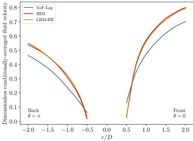
Figure 14: Dimensionless conditionally-averaged fluid velocity for t = 1.25T_e^0 (1s) along the axis.
