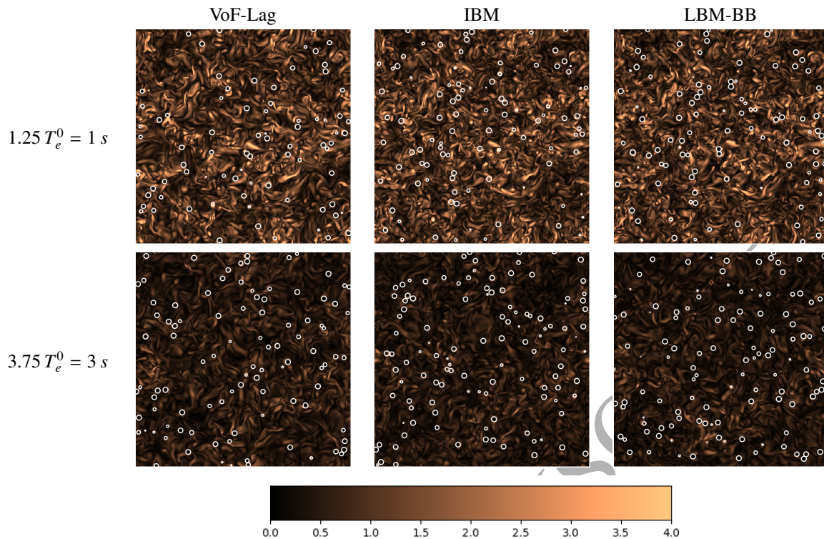
Figure 7: Vorticity field for the x - y plane and z = 0 obtained with each method for the 512^3 case. The vorticity magnitude is divided by the averaged value for t = 1.25 T_e^0 = 1 s .
