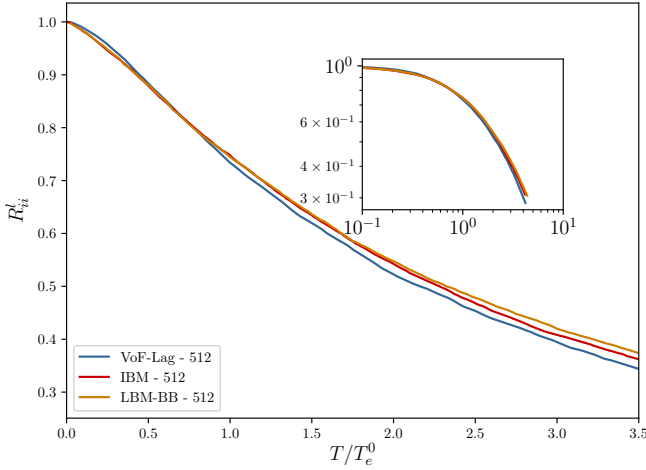
Figure 11: Lagrangian velocity autocorrelation function starting at t_0 = 1.25 T_e^0 = 1 s .
