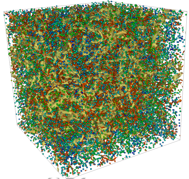
Figure 4: Visualization of particle-laden decaying HIT. Particles are colored by their linear velocity (green-high and blue-low). Red denotes iso-surfaces of constant Q -criterion, while translucent yellow represents iso-surfaces of low pressure regions. Case 1024 simulated with IBM code, at time 1.25 T_e^0 = 1 s.
