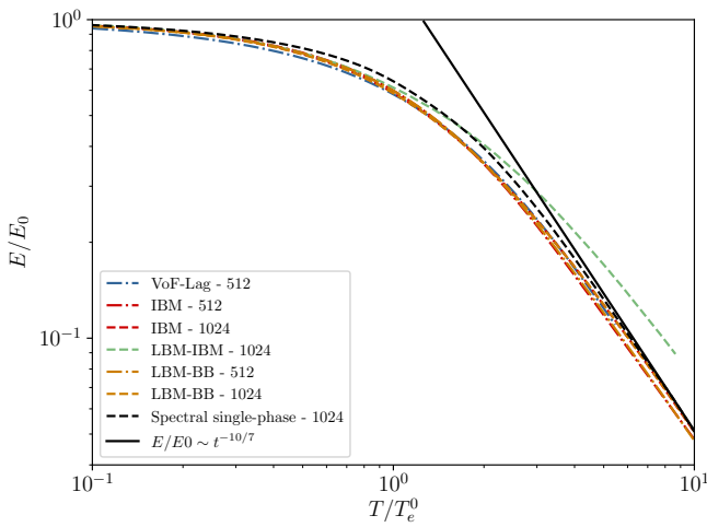
Figure 8: Decaying fluid kinetic energy of two-phase flow. E_0 and T_e^0 denote the values of kinetic energy and eddy turnover time at T = 0 , respectively.
