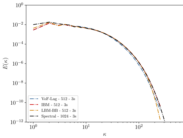
Figure 6: Spectra for single-phase case for two given times. Top: t = 1.25T_e^0 (1 s); Bottom: t = 3.75T_e^0 (3 s).
