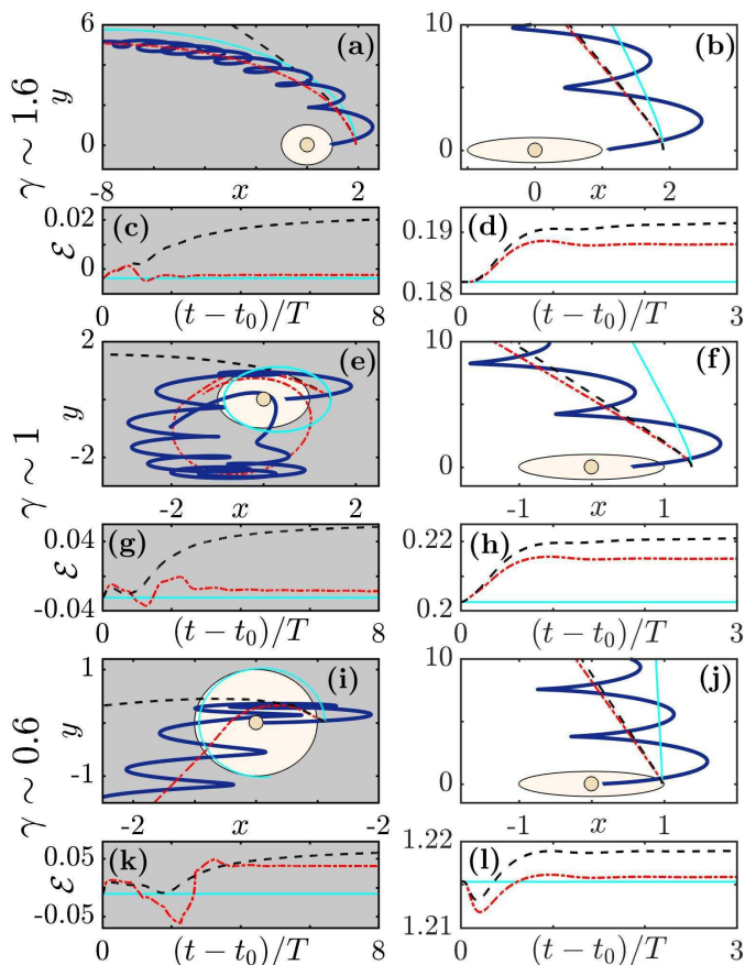
FIG. 12: (a,b,e,f,i,j) T-trajectory in the polarization plane ( x, y ). The thick dark blue curves are the T-trajectory of the reference Hamiltonian. The red dash-dotted, cyan solid and dashed black curves are the T-trajectory of Hamiltonian (6), the GC model (12) and the CCSFA (9), respectively. (c,d,g,h,k,l) Energy (12) as a function of (t - t_0)/T , with t_0 = T/2 , associated with each model. Right panels: \xi = 0.7 . (a,c), (e,g) and (i,k) (the grey background panels are those for \xi < \xi_c ) \xi = 0.25 , \xi = 0.15 and \xi = 0.05 , respectively. (a-d) are for I = 8 \times 10^{13} \text{ W} \cdot \text{cm}^{-2} , He ( I_p = 0.9 \text{ a.u.} ) and \gamma \sim 1.6 (same parameters as the top panels of Fig. 11). (e-h) are for I = 1.2 \times 10^{14} \text{ W} \cdot \text{cm}^{-2} , Ar ( I_p = 0.58 \text{ a.u.} ) and \gamma \sim 1 (same parameters as the middle panels of Fig. 11). (i-l) are for I = 8 \times 10^{14} \text{ W} \cdot \text{cm}^{-2} , He ( I_p = 0.9 \text{ a.u.} ) and \gamma \sim 0.6 (same parameters as the lower panels of Fig. 11). The dots indicate the origin, and the circles |\mathbf{r}| = E_0/\omega^2 . The distances are scaled by E_0/\omega^2 .
