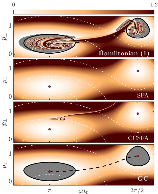
FIG. 3: Electron final energy as a function of the initial conditions ( t_0, p_\perp, p_\parallel = 0 ) for I = 8 \times 10^{13} \text{ W} \cdot \text{cm}^{-2} and \xi = 0.4 of the reference Hamiltonian (1), the SFA [1, 13], the CCSFA [17] and the GC model (12). In grey-colored regions, the electron final energy is negative. The white dashed lines are contours of constant ionization rate W(t_0, p_\perp) (see Appendix A) for W/\max(W) = 10^{-1}, 10^{-5} and 10^{-15} , from bottom to top. The red dots correspond to the initial conditions for which the electron final energy in the SFA is zero, i.e., \mathcal{E}^{\text{SFA}} = 0 [see Eq. (14)]. The solid black lines correspond to the initial conditions for which the GC energy is zero, i.e., \mathcal{E} = 0 [see Eq. (15)]. The black dashed line corresponds to the initial conditions for which the GC angular momentum is zero and the initial radial momentum is negative, i.e., \mathbf{L} = \mathbf{0} and p_r(t_0) < 0 , where \mathbf{L} = \bar{\mathbf{r}}_g \times \bar{\mathbf{p}}_g and p_r = \bar{\mathbf{p}}_g \cdot \bar{\mathbf{r}}_g / |\bar{\mathbf{r}}_g| . The momentum and the energy are scaled by E_0/\omega and U_p = E_0^2/4\omega^2 , respectively.
