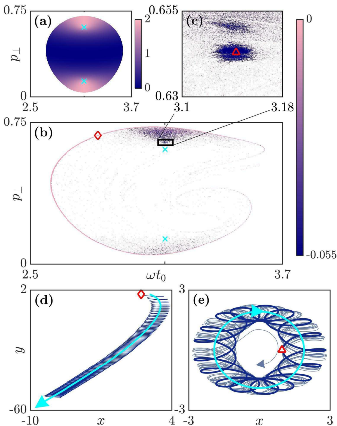
FIG. 7: The parameters are I = 8 \times 10^{13} \text{ W} \cdot \text{cm}^{-2} , \xi = 0.4 and plateau duration T_p = 100T . (a) GC perihelion [see Eq. (B1)] in the rescattering domain depicted in the space of initial conditions (t_0, p_\perp, p_\parallel) . (b) Final negative energies of the electron trajectories of the reference Hamiltonian (1), where (c) is a zoom around the trapping region. The white color in (a–c) denotes an electron not trapped at the end of the laser pulse. (d),(e) Trajectories for the initial conditions indicated with a diamond in (c) and a triangle in (b), respectively. The dark blue and cyan curves are the electron trajectory of the reference Hamiltonian (1) and the GC trajectory, respectively. The thick dark blue curve in (e) is a center-saddle periodic orbit very close to the region depicted in (c). The cyan crosses in (a) and (b) are the initial conditions of the clockwise (upper cross) and anticlockwise (lower cross) circular GC orbits. The cyan curve in (e) is the GC clockwise circular orbit, whose initial conditions are very close to the trapping region depicted in (c). Momenta and distance are scaled by E_0/\omega and E_0/\omega^2 , respectively.
