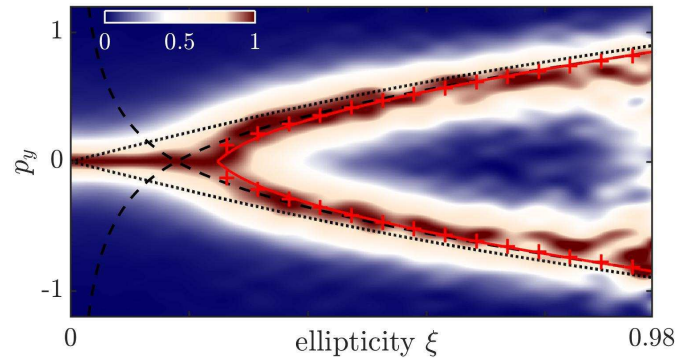
FIG. 10: Photoelectron momentum distribution along the minor polarization axis \hat{y} as a function of the ellipticity for I = 1.2 \times 10^{14} \text{ W} \cdot \text{cm}^{-2} and Ar ( I_p = 0.58 \text{ a.u.} ) and \gamma \sim 1 . The color scale is the experimental data of Ref. [26]. The dotted and dashed black lines are the T-trajectory of the SFA and the CCSFA, respectively. The cross markers and red solid lines are the T-trajectory of the reference Hamiltonian (1) and the GC model (12), respectively. Momenta are scaled by E_0/\omega .
