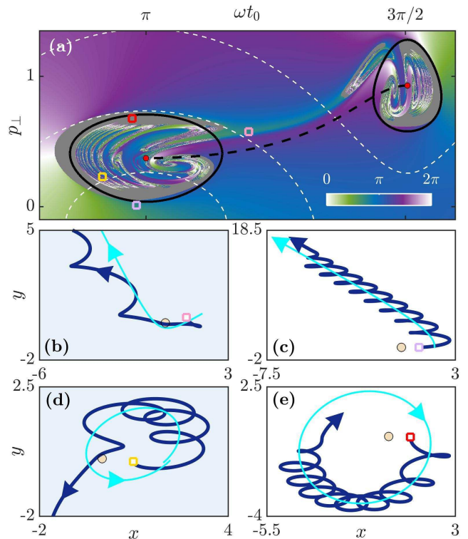
FIG. 4: (a) Scattering angle of the electron as a function of the initial conditions after tunneling (t_0, p_\perp, p_\parallel = 0) for I = 8 \times 10^{13} \text{W} \cdot \text{cm}^{-2} and \xi = 0.4 . The white dashed lines are the contours of constant ionization rate W(t_0, p_\perp) (see Appendix A) for W/\max(W) = 10^{-1}, 10^{-5} and 10^{-15} , from bottom to top. The red dots correspond to the initial conditions for which \mathcal{E}^{\text{SFA}} = 0 [see Eq. (14)]. The solid black line corresponds to the initial conditions for which \mathcal{E} = 0 [boundaries of the rescattering domain for the GC model, see Eq. (15)]. The black dashed line corresponds to the initial conditions for which the GC angular momentum is zero and the initial radial momentum is negative, i.e., \mathbf{L} = \mathbf{0} and p_r(t_0) < 0 , where \mathbf{L} = \mathbf{r}_g \times \mathbf{p}_g and p_r = \mathbf{p}_g \cdot \mathbf{r}_g/|\mathbf{r}_g| . Grey areas show the conditions for which the electron is trapped into Rydberg states. (b–e) Dark and light blue curves are the electron and its GC trajectory, respectively. The initial condition of each trajectory is associated with a marker represented in (a). These trajectories represent a typical: (b) subcycle recollision, (c) direct ionization, (d) Coulomb-driven recollision, and (e) Rydberg state creation. Panels (b) and (c) have positive GC energy, while (d) and (e) have negative GC energy. Blue shaded panels indicate the cases with recollisions. The momentum and position are scaled by E_0/\omega and E_0/\omega^2 , respectively.
