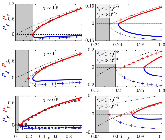
FIG. 11: Final momentum of the T-trajectory \mathbf{P} = P_x \hat{x} + P_y \hat{y} as a function of the ellipticity \xi . Top panels: I = 8 \times 10^{13} \text{ W} \cdot \text{cm}^{-2} , He ( I_p = 0.9 a.u.) and \gamma \sim 1.6 . Middle panels: I = 1.2 \times 10^{14} \text{ W} \cdot \text{cm}^{-2} , Ar ( I_p = 0.58 a.u.) and \gamma \sim 1 . Bottom panels: I = 8 \times 10^{14} \text{ W} \cdot \text{cm}^{-2} , He ( I_p = 0.9 a.u.) and \gamma \sim 0.6 . The hexagrams are the experimental data reproduced from Ref. [18]. In all panels: the dotted and dashed black lines are the T-trajectory of the SFA and the CCSFA, respectively. The thin (with crosses) and solid curves are the T-trajectory of the reference Hamiltonian (1) and the GC model (12), respectively. The components of the final momentum of the T-trajectory P_x and P_y are depicted in blue and red, respectively. The critical ellipticity \xi_c is at the intersection between the grey and white regions and corresponds to the largest ellipticity for which the T-trajectory of the reference Hamiltonian (1) is negative. The right panels are zooms of the left panels in the neighborhood of the critical ellipticity. We indicate the scaling of \mathbf{P} of the reference model (1) in the neighborhood of the bifurcation. Momenta are scaled by E_0/\omega .
