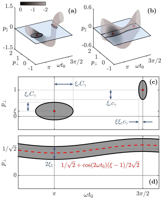
FIG. 9: Shape of the rescattering domain for I = 8 \times 10^{13} \text{ W} \cdot \text{cm}^{-2} and \xi = 0.2 [close to LP, (a) and (c)], and \xi = 0.7 [close to CP, (b) and (d)]. (a), (b) Boundary of the rescattering domain as a function of the initial conditions (t_0, p_{\parallel}, p_{\perp}) . The color is the logarithm of the PPT ionization rate normalized by its maximum. The black lines are the boundaries of the rescattering domain for p_{\parallel} = 0 . (c), (d) Slice of the initial conditions p_{\parallel} = 0 [shaded blue planes in (a) and (b)]. Only the dominant orders in \xi are depicted. Momenta are scaled by E_0/\omega .
