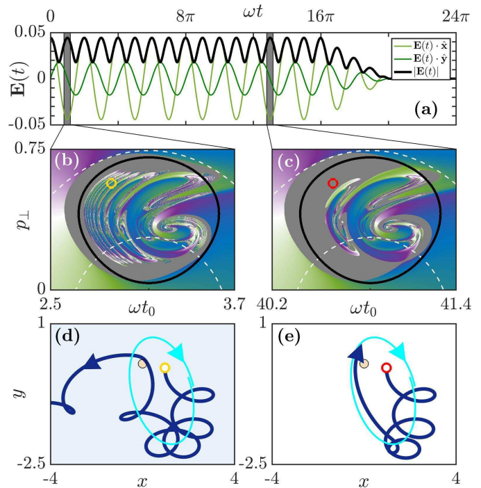
FIG. 5: (a) Electric field components and amplitude as a function of \omega t . The grey regions indicate the ionization time for which the final scattering angle is computed in (b) and (c). (b-c) Final scattering angle of the ionized electron as a function of the initial conditions ( \omega t_0, p_\perp, p_\parallel = 0 ) for I = 8 \times 10^{13} \text{ W} \cdot \text{cm}^{-2} and \xi = 0.4 for the reference Hamiltonian (1). The white dashed lines are the contour plot of the ionization rate W(t_0, p_\perp) (see Appendix A) for W/\max(W) = 10^{-1}, 10^{-5} and 10^{-15} , from bottom to top. The solid black line corresponds to the initial conditions for which \mathcal{E} = 0 [boundaries of the rescattering domain for the GC model, see Eq. (15)]. The dark grey region corresponds to the initial conditions for which the electron is trapped into a Rydberg state at the end of the pulse. (d-e) Dark and light blue curves are the electron and its GC trajectory, respectively. The initial conditions of the trajectories in (d) and (e) are indicated by circles in (b) and (c), respectively. The trajectories in (d) and (e) are initialized at the same laser phase, but (d) is a Coulomb-driven recollision and (e) is a Rydberg state creation. The momentum and the position are scaled by E_0/\omega and E_0/\omega^2 , respectively.
