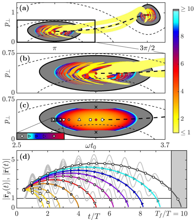
FIG. 6: Recollisions in the GC model for I = 8 \times 10^{13} \text{ W} \cdot \text{cm}^{-2} and \xi = 0.4 . (a) \Delta t/T as a function of the initial conditions (t_0, p_\perp, p_\parallel = 0) , where \Delta t is the smallest time interval such that |\bar{\mathbf{r}}(t_0 + \Delta t)| = 5 \text{ a.u.} , with t_0 + \Delta t < T_f (laser pulse duration T_f = 10T ) and \bar{\mathbf{r}}(t) = \bar{\mathbf{r}}_g(t) + \boldsymbol{\Sigma}(t)/\omega^2 (reconstructed trajectory). The white and dark grey regions are where this condition is never met, and where the GC energy is positive (white region) and negative (grey region). (b) Zoom of (a) on the largest rescattering domain. (c) T_g/T = \omega/(2|\mathcal{E}|)^{3/2} . The dark grey region is where the GC perihelion [see Eq. (B1)] is greater than the quiver radius E_0/\omega^2 \approx 14 \text{ a.u.} , or where t_0 + T_g \geq T_f . The inset is a zoom. (a–c) The red dots and the black thick dashed curves are the same as in Fig. 3a. (c) The crosses are the location of the GC circular orbits (see Sec. IV B). The dark dashed lines are contours of constant ionization rate W(t_0, p_\perp) (see Appendix A) for W/\max(W) = 10^{-1}, 10^{-5} and 10^{-15} , from bottom to top. (d) The lines with markers are the GC trajectories |\bar{\mathbf{r}}_g(t)| with initial conditions plotted in panel (c) with the corresponding marker and color, and the light grey lines are the reconstructed trajectories |\bar{\mathbf{r}}(t)| . The light grey region is when the laser field is turned off. Momenta are scaled by E_0/\omega .
