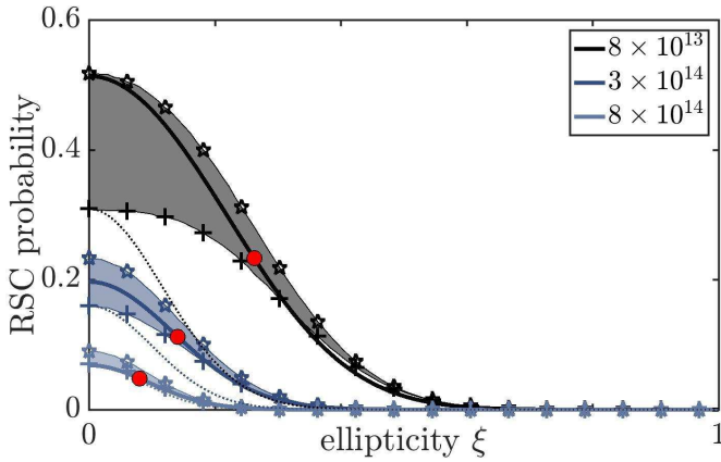
FIG. 8: Rydberg state creation (RSC) probability as a function of the laser ellipticity \xi for I = 8 \times 10^{13} , 3 \times 10^{14} , and 8 \times 10^{14} \text{W} \cdot \text{cm}^{-2} . The RSC probability is defined as the ratio of the RSC yield \mathbb{Y} to the ionized electron yield N = \int_0^{T_f} dt_0 \int_{-\infty}^{\infty} d^2\mathbf{p}_0 W(t_0, \mathbf{p}_0) . The thick solid and dotted curves are our prediction with the GC model \mathbb{Y}_{\text{GC}}/N [Eq. (18)], and the SFA \mathbb{Y}_{\text{SFA}}/N , respectively. The thin curves with stars and crosses are the CTMC simulations of the reference Hamiltonian (1) using T_p = T and T_p = 8T , respectively. The filled areas show the estimate of the Coulomb-driven recollision probability for T_p = 8T . Red circles show the probability of RSC at the critical ellipticity \xi_c given by Eq. (22).
