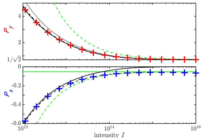
FIG. 1: T-trajectory final momentum \mathbf{P} = P_x \hat{\mathbf{x}} + P_y \hat{\mathbf{y}} as function of the laser intensity I for \xi = 1 . The crosses are the T-trajectory final momentum of the reference Hamiltonian (1), where P_x and P_y are in blue and red, respectively. The dotted, dashed and solid black curves are the T-trajectory final momentum of the SFA, the CCSFA and the GC model, respectively. The dashed and solid green lines are the approximated and the asymptotic T-trajectory final momentum using Eqs. (10) and (13), respectively. Momenta are scaled by E_0/\omega .
