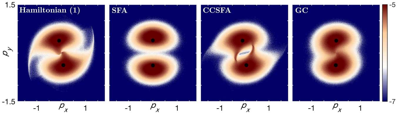
FIG. 2: Photoelectron momentum distributions (PMDs) in logarithmic scale for I = 8 \times 10^{13} \text{ W} \cdot \text{cm}^{-2} and \xi = 0.4 of the reference Hamiltonian (1), the SFA [1, 13], the CCSFA [17] and the GC model. The upper (resp. lower) black dot is the T-trajectory final momentum for each model (resp. its symmetric momentum with respect to the origin). The momenta are scaled by E_0/\omega .
