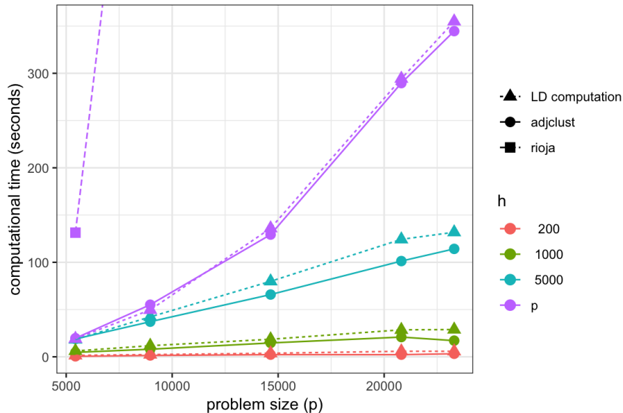
Figure 7: Computation times versus p : LD matrices, for CHAC rioja and adjclust with varying values for the band h .
