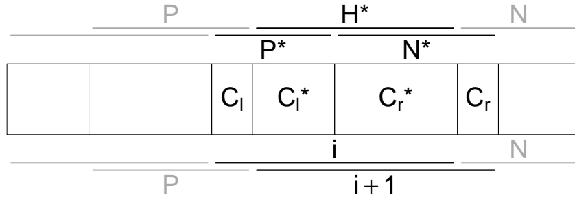
Figure 4: Illustration of the result of a merging step in Algorithm 2.
