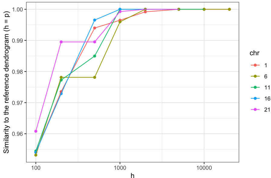
Figure 6: Quality of the band approximation as a function of the bandwidth h for five different chromosomes.
