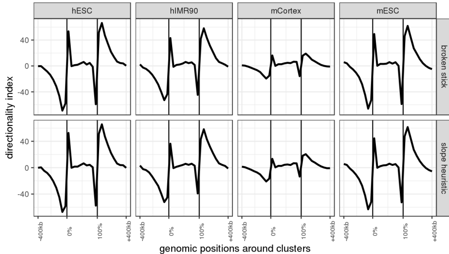
Figure 9: Evolution of the Directionality Index (DI) around clusters.
