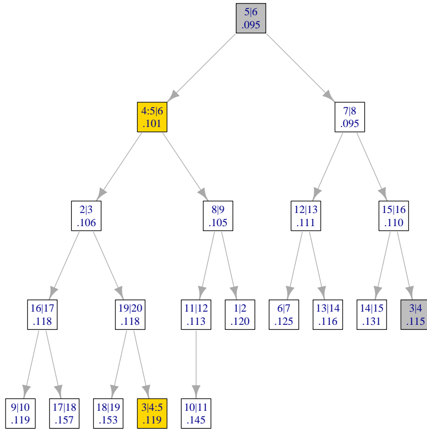
Figure 5: Min heap after the first merging step for the RLGH data set. The nodes corresponding to the fusion that have changed since initialization (Figure 3) are highlighted.
