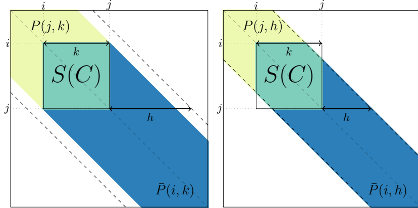
Figure 1: Example of forward pencils (in yellow and green) and backward pencils (in green and blue), and illustration of Equation (3) for cluster C = \{i, \dots, j - 1\} . Left: cluster smaller than bandwidth ( k \leq h ); right: cluster larger than bandwidth k \geq h .
