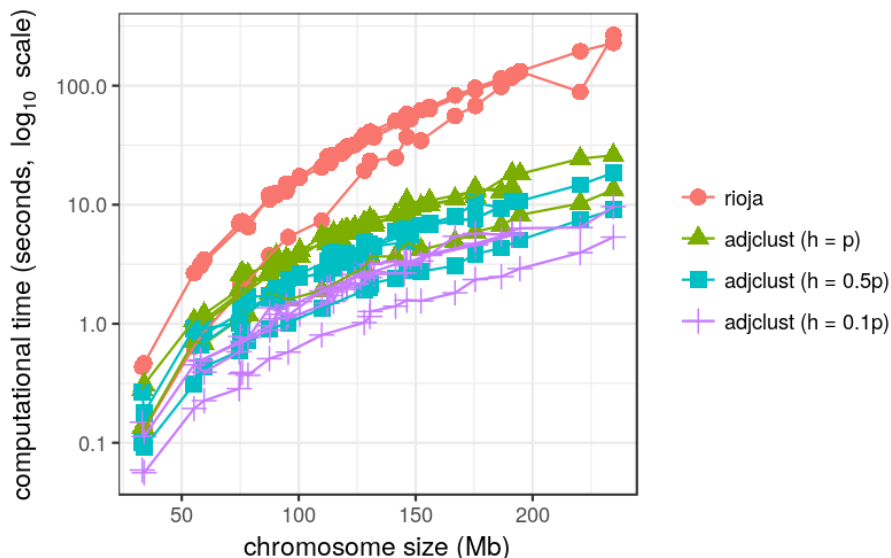
Figure 8: Impact of sparsity on the computational time. Dots that correspond to the same datasets but different chromosomes are linked by a path.
