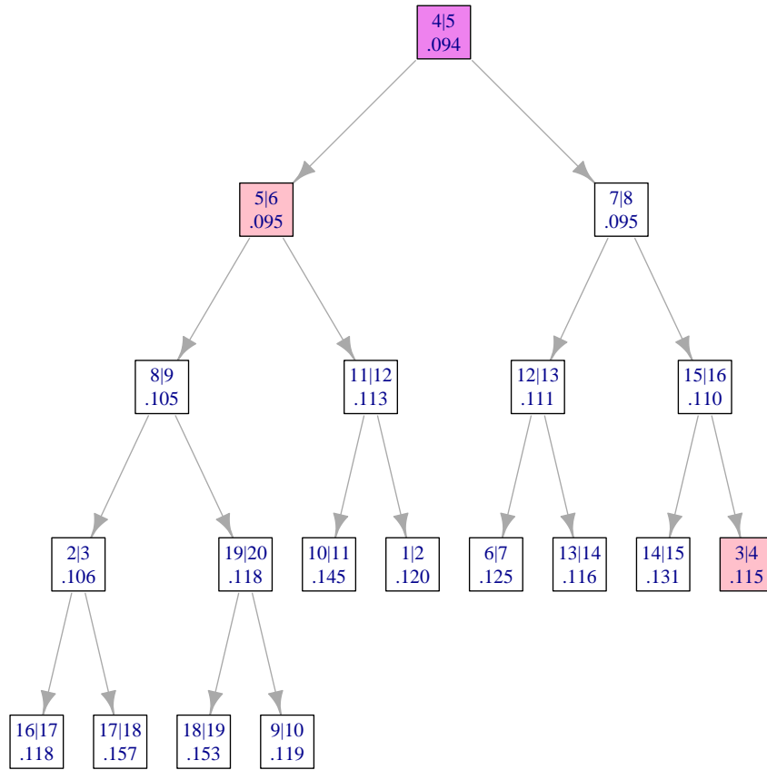
Figure 3: Min heap after the initialization step of the RLGH data set. Each node corresponds to a candidate fusion, and is represented by a label of the form i|i + 1 giving the indices of the items to be merged, and (ii) the value of the corresponding linkage \delta(\{i\}, \{j\}) . The nodes corresponding to the best fusion and the two neighbor fusions are highlighted.
