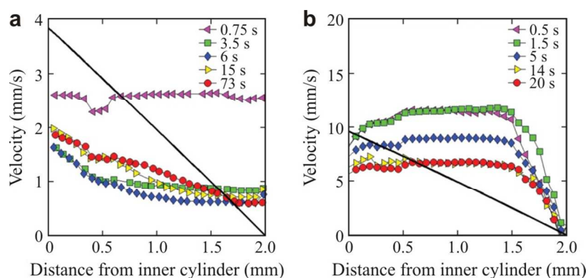
Figure 9 Height average velocity profiles at different times of applied shear for (a) enzymatically hydrolyzed CNF suspension at a concentration of 2 wt.%, applied shear rate of 2 \text{ s}^{-1} and (b) TEMPO-oxidized CNF suspension at a concentration of 1 wt.%, applied shear rate of 5 \text{ s}^{-1} . On the abscissa axis, 0 and 2 mm correspond to inner and outer Couette surfaces, respectively. Solid lines represent a theoretical profile at a given shear rate in case of laminar flow (adapted from ref. 33 . Copyright 2015, with permission of The Royal Society of Chemistry. http://dx.doi.org/10.1039/c5sm00530b ).
