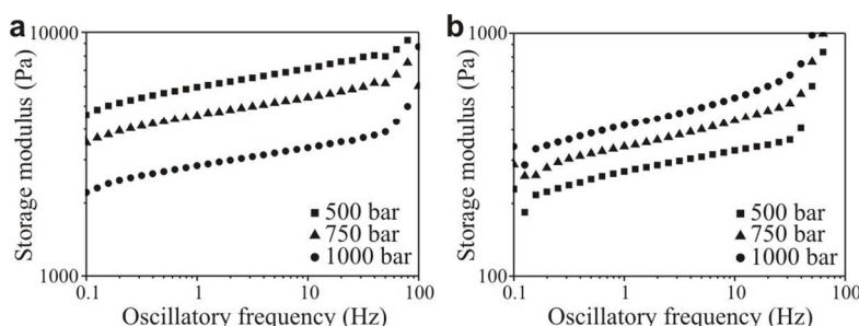
Figure 3 Storage modulus of enzymatically hydrolyzed CNF suspensions at 2 wt.% produced using homogenization at different applied pressures (a) without preshear and (b) with preshear protocol (adapted from ref. 36 . Copyright 2015, with permission from Nova Science Publishers, Inc.).
