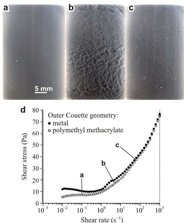
Figure 6 Photographs showing a structure of mechanically fibrillated CNF suspensions at 1 wt.% at the outer Couette surface at the shear rates of 0.1 s -1 (a), 5.0 s -1 (b) and 63.1 s -1 (c); the inner cylinder rotates to the left; and the corresponding flow curves (d) measured using geometries with different outer geometry surfaces (adapted from ref. 75 . Copyright 2012 Springer Science+Business Media B.V. With permission of Springer).
