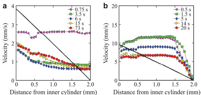
19 20 21 22 23 24 25 26 27 28 29 30 31 32 33 Figure 9 Height average velocity profiles at different times of applied shear for (a) 34 35 enzymatically hydrolyzed CNF suspension at a concentration of 2 wt.%, applied shear rate of 36 37 2 \text{ s}^{-1} and (b) TEMPO-oxidized CNF suspension at a concentration of 1 wt.%, applied shear rate 38 39 of 5 \text{ s}^{-1} . On the abscissa axis, 0 and 2 mm correspond to inner and outer Couette surfaces, 40 41 respectively. Solid lines represent a theoretical profile at a given shear rate in case of laminar 42 43 flow (adapted from ref. 33 . Copyright 2015, with permission of The Royal Society of Chemistry. 44 45 http://dx.doi.org/10.1039/c5sm00530b ). 46 47 48 49 50 51 52 53
