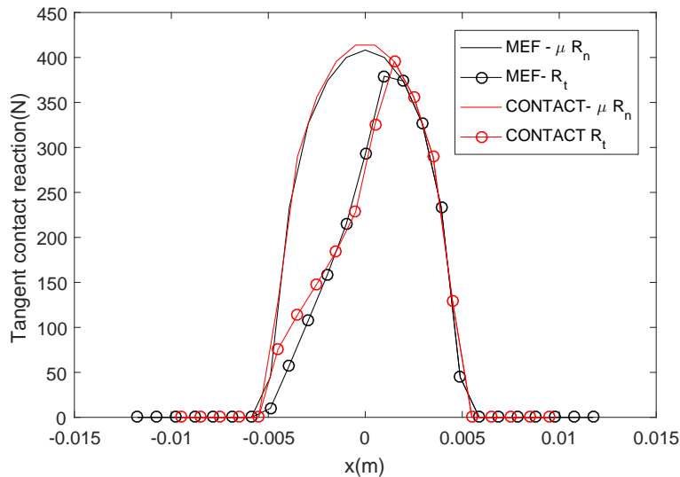
FIGURE 4 – Tangent contact reaction at y = 0
