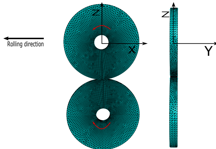
FIGURE 2 – Contact between 2 cylinders
