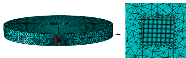
FIGURE 3 – Mesh of the 2 cylinders with discretization of the contact surface
