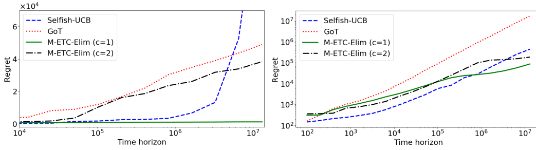
Figure 2: Numerical comparison of M-ETC-Elim, GoT and Selfish-UCB on reward matrices U_1 (left) and U_2 (right) with Gaussian rewards and variance 0.05. The x-axis has logarithmic scale in both plots. The y-axis has logarithmic scale in the right plot.
