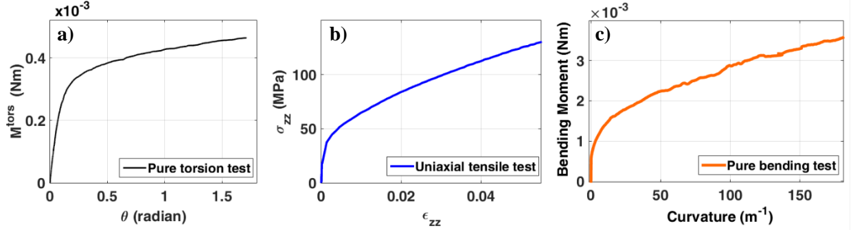
Figure 1. Input experimental data on pure copper wire ( \phi=0.6\text{mm} ) (a) Pure torsion test results, (b) Pure uniaxial tensile test results, (c) Pure bending test results.
