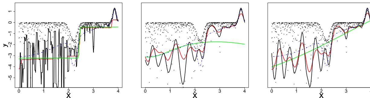
Figure 20: Metamodel responses for toy problem 3 and \tau = 0.1 with 640 training sample (left: RF, center: RK, right: VB) for different values of hyperparameters. The true 0.1-quantile is presented in dotted blue lines. In green and black two extreme metamodels associated to two extreme hyperparameter values, while in red the oracle metamodels are represented.
