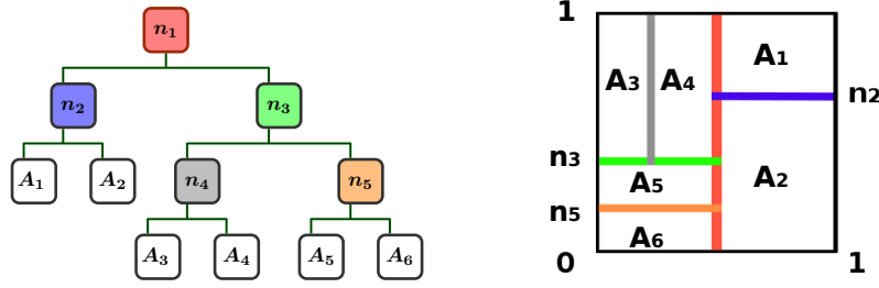
Figure 2: Left: a partitioning tree T . The nodes n_i ( 1 \leq i \leq 5 ) represent the splitting points, the A_i 's ( 1 \leq i \leq 6 ) represent the leaves. Right: \mathcal{X} = [0, 1]^2 as partitioned by T . The regression tree prediction is constant on each leaf A_i .
