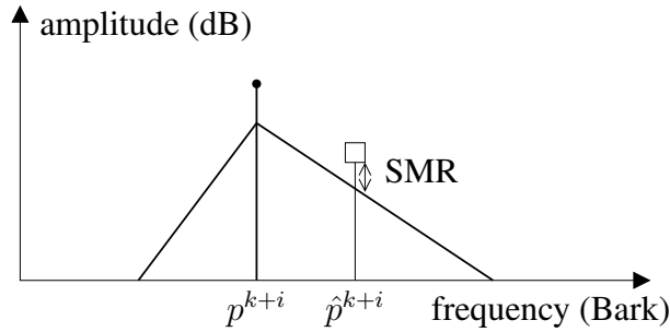
Figure 3: Frequency masking curve.
