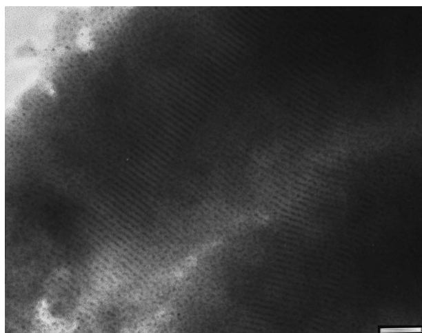
Figure 18 Au nanoparticles within the channels of thiol functionalised ordered mesoporous silica (scale bar = 50 nm).
