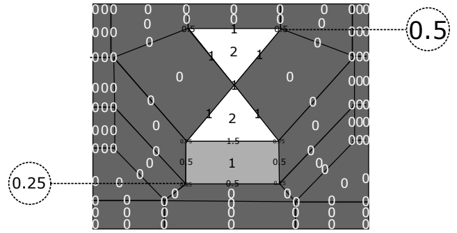
Fig. 14: Flattening of U_{\text{USC}} into u^b : Y \rightarrow \mathbb{R} using the symmetric median operator.
