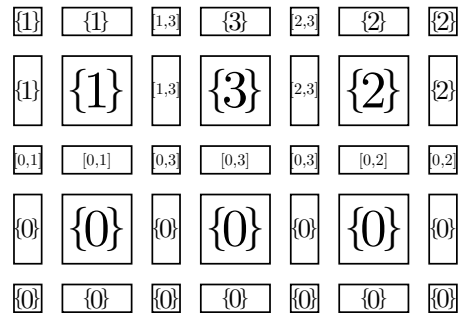
Fig. 8: An example of span-valued map on a 2D Khalimsky grid. Observe that this map is “flat” on the squares and that the values on the vertices and edges depend only on the values of U on the squares which contain them.
