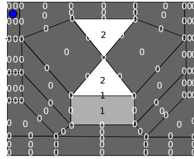
Fig. 17: Flattening of U_{\text{USC}} into u^b : Y \rightarrow \mathbb{R} thanks to the front propagation algorithm.
