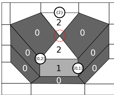
Fig. 12: The initial image U : X \rightarrow \mathbb{I}_{\mathbb{R}} , containing a pinch encircled in red: at this vertex, the boundary of [U \triangleright 1] crosses itself. Circles indicate the values of the span-valued map U on some of the k -faces of X ( k < n ).
