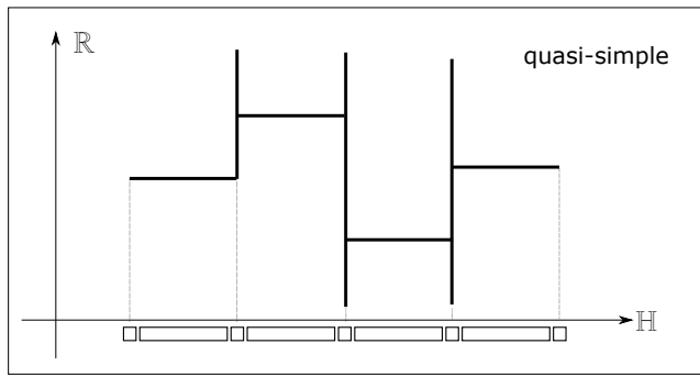
Fig. 24: An example of quasi-simple map on the 1D Khalimsky grid \mathbb{H} : we can observe that this map U is USC, that for any x in the domain of U , the set U(x) is connected and closed, and that U(x) is “flat” on the maximal faces.
