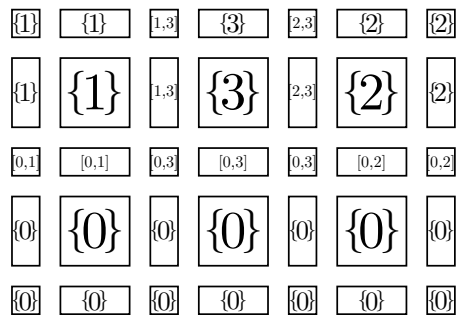
Fig. 8: An example of span-valued map on a 2D Khalimsky grid. Observe that this map is “flat” on the squares and that the values on the vertices and edges depend only on the values of U on the squares which contain them.
