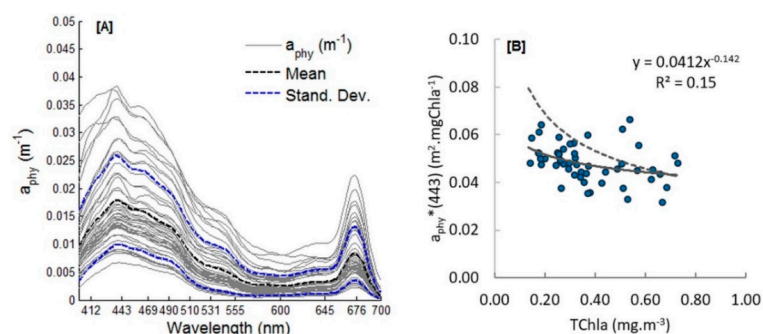
Figure 4. Phytoplankton absorption ( a_{\text{phy}} ) spectra (A) and specific phytoplankton absorption coefficient ( a_{\text{phy}}^* ) at 443 nm versus the TChl a , with the power law regression fit (solid line) and the Bricaud et al. [23] fit for reference (dashed line) (B) (Number of samples = 52).
