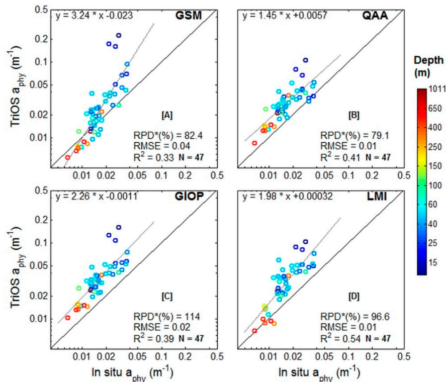
Figure 12. Comparisons between the in situ measured and modelled phytoplankton absorption ( a_{phy} ) at 443 nm using Remote sensing reflectance from TriOS radiometer ( R_{rs}T ) (TriOS a_{phy} ) obtained with: Garver-Siegel-Maritorena (GSM01) (A), Quasi-Analytical Algorithm (QAA) (B), Generalized IOP (GIOP) (C) and Linear Matrix Inversion (LMI) (D) (Number of samples = 47). Axes in log scale.
