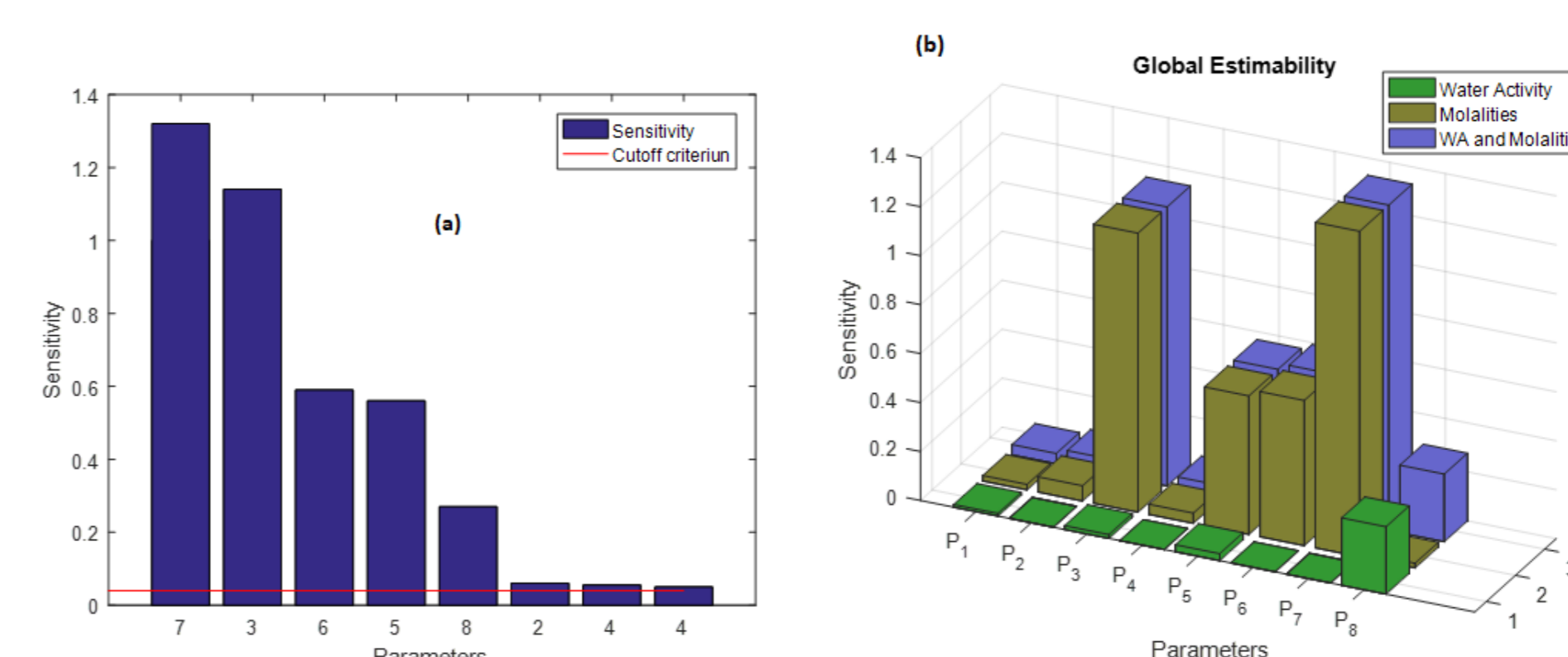
Figure: a: Estimability using all experimental measurements, b: Estimability for all cases
