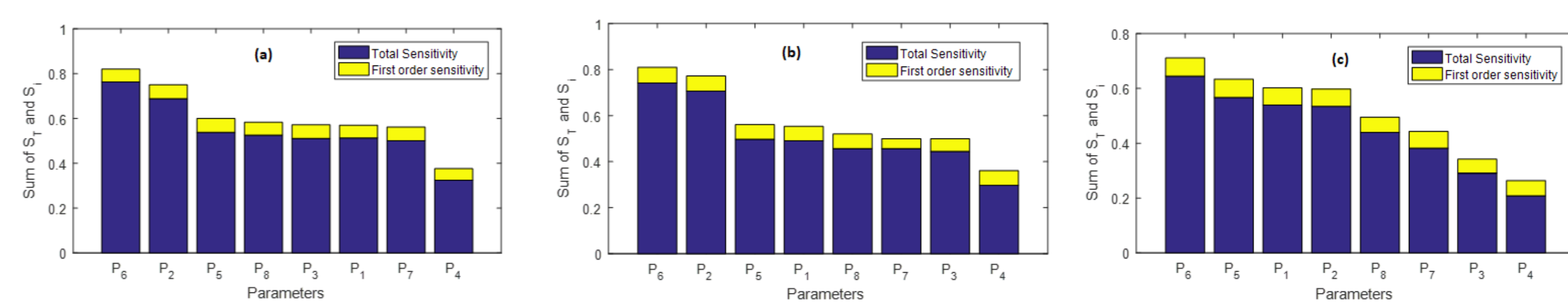
Figure: S_T and S_i for H^+ molality, a: C=6moles/Kg, b: C=3 moles/Kg, c: C=1mole/Kg
