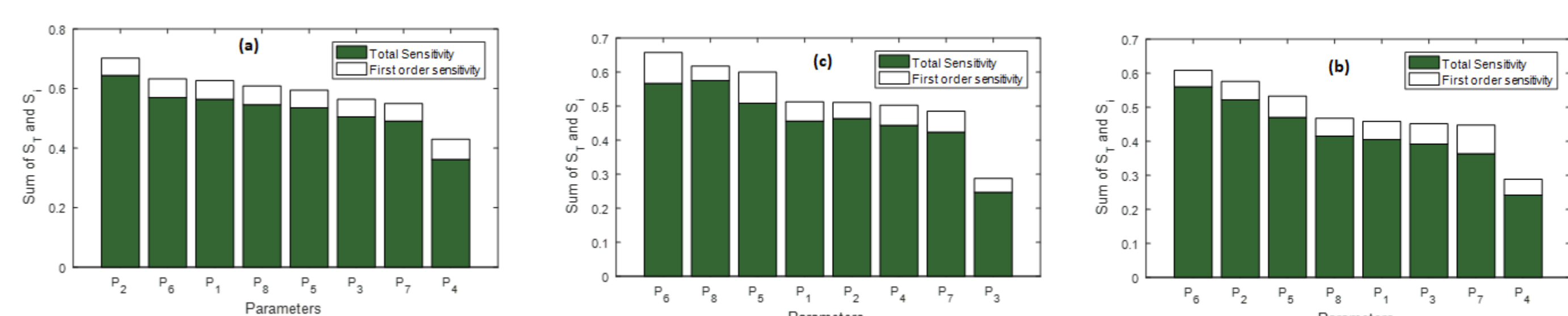
Figure: S_T and S_i for HSO_4^- molality, a: C=6moles/Kg, b: C=3 moles/Kg, c: C=1mole/Kg
