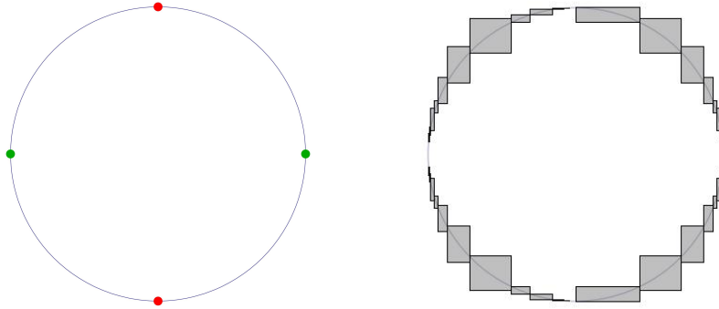
Fig. 2. Left: The \underline{\text{PR}}\text{-RP} kinematic model solutions set. Right: The computed paving.
