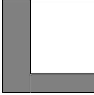
Figure 5: The n \times m strong grid with the area in white representing the a \times b subgrid and the area in gray representing the remaining rows and columns.
