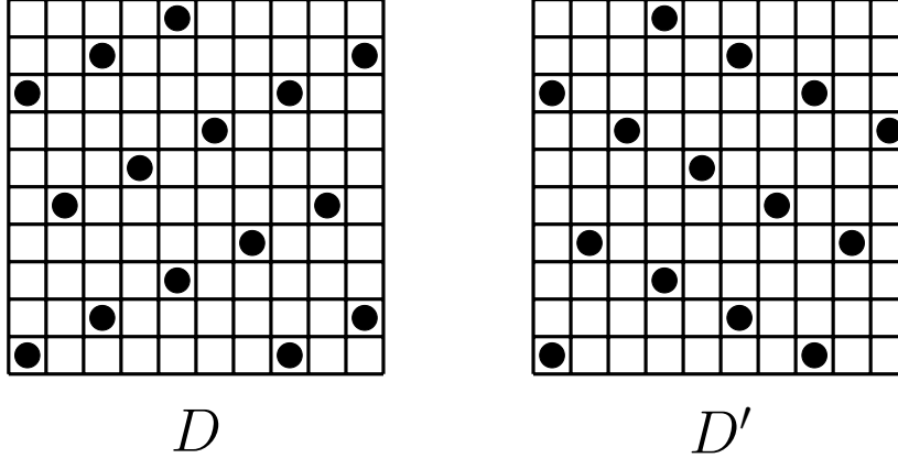
Figure 2: Snapshot of a 10 \times 10 subgrid of a much larger grid, showing the positions of the guards in a D (left) and a D' (right) configuration.
