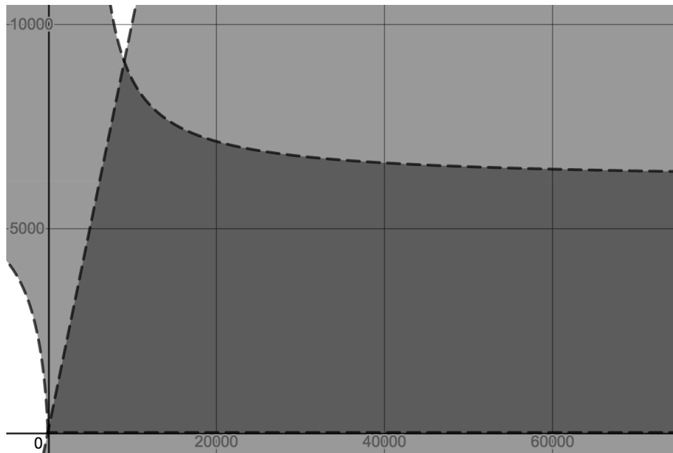
Figure 6: Comparison of bounds (1) and (2); m as horizontal axis, n as vertical axis
