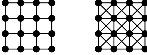
Figure 1: The cartesian grid P_4 \square P_4 (left) and strong grid P_4 \boxtimes P_4 (right).
