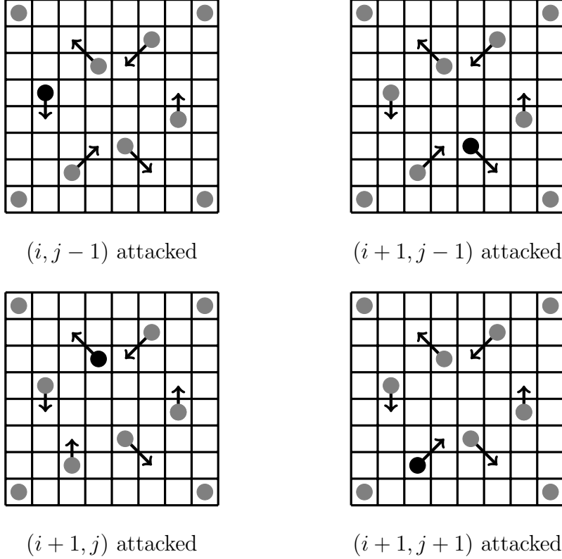
Figure 3: Movements of guards from a D to a D' configuration in the 8 \times 8 subgrid corresponding to all possible attacks (less symmetric cases). The black guard occupies vertex (i, j) and the four anchor guards are the guards in the corners.
