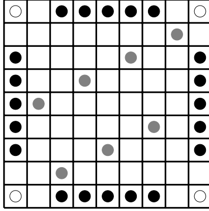
Figure 4: One possible configuration of the guards in the 9 \times 9 strong grid with the guards in white in the corners never moving, the guards on the paths of length 7 between the corners in black, and the remaining guards in gray.
