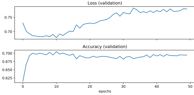
Fig. 2. Averaging the 4 cases loss (top) and accuracy (bottom) on development set after each epoch on the SNN architecture.
