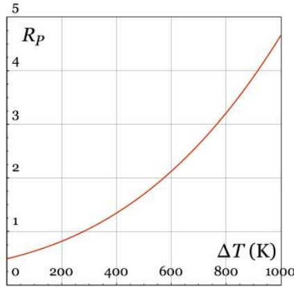
Figure 23: Variation of R_P as a function of \Delta T . The larger the temperature difference, the more important becomes radiative transfer compared to free convection.
