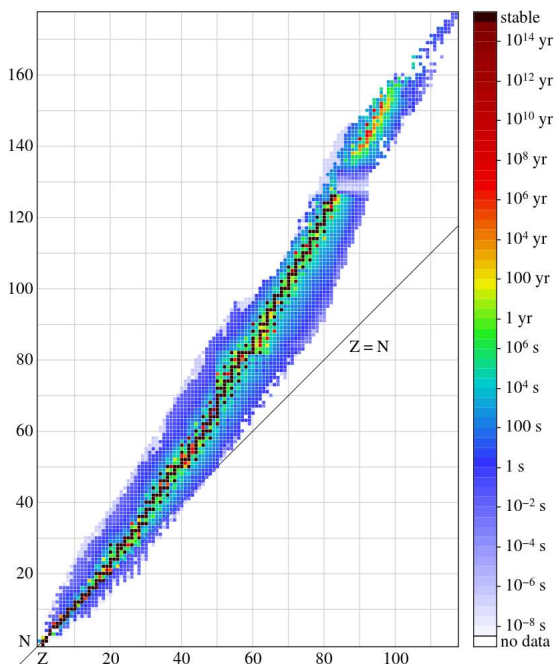
Figure 7: Plot of atomic isotopes (Z: number of protons, N: number of neutrons) colored by half life. From [26]
