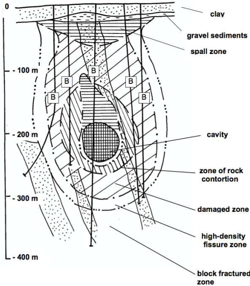
Figure 13: Same kind of diagram as Fig. 12 but for a real nuclear test in former USSR (Balapan test site). From [34], p. 12, Fig. 4.
