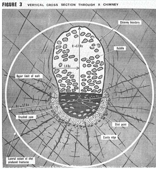
Figure 12: Vertical cross section through a chimney resulting from a deep underground nuclear explosion. From [39].
