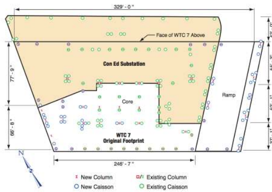
Figure 5-1 Foundation plan - WTC 7.
