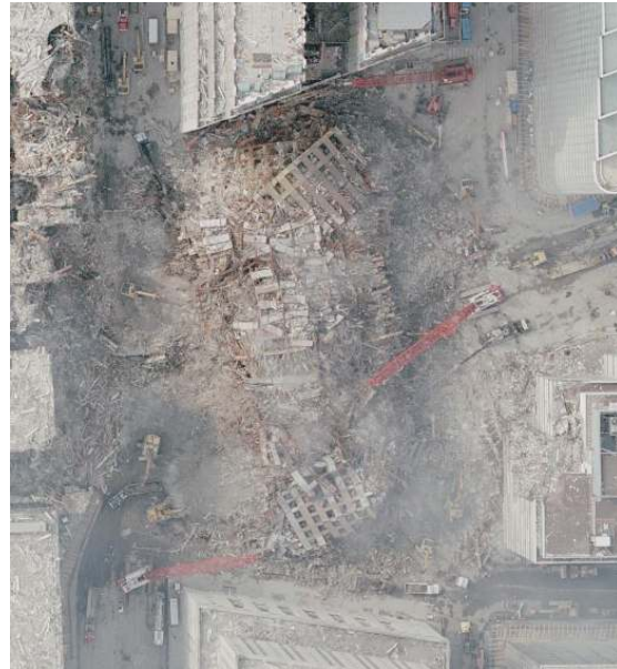
Figure 18: Aerial picture of WTC7 rubble pile during cleanup operation, cropped from [55]. Some almost undamaged facade walls parts are clearly visible, covering some much more shattered debris.
