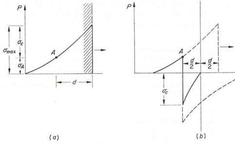
FIGURE 2.11 Spallation will occur when the wave penetrates a distance d/2 into the interface then the tension on the material equals \sigma_c .
