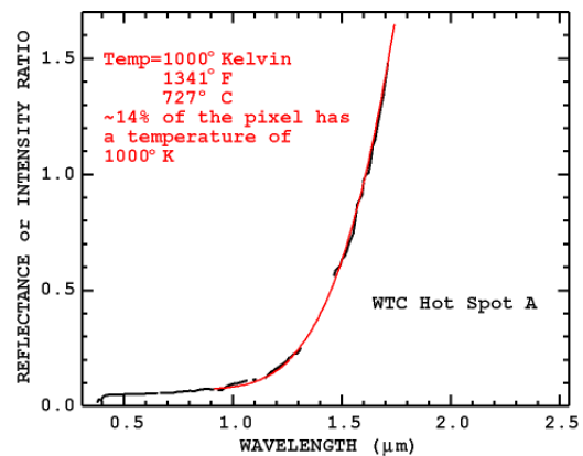
Figure 2: Example of IR radiation spectral analysis for surface temperature determination, as explained in [23]. The area at 1000 K (on September 16, 2001) covers 0.56 \text{ m}^2 according to authors and is located in the WTC7 debris.
