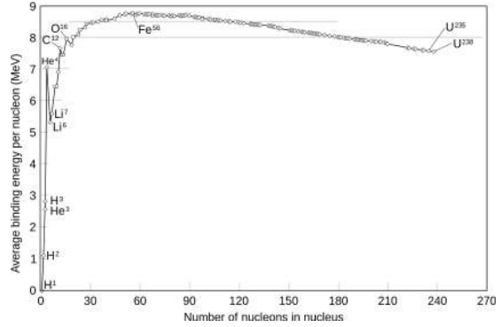
Figure 9: Average binding energy per nucleon in MeV against number of nucleons in nucleus, for relatively abundant isotopes. From [29]
