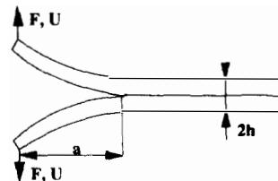
Fig. 7. DCB test.
