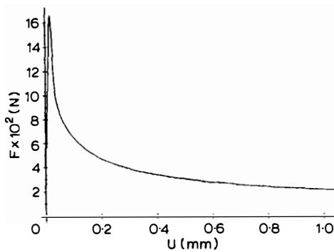
Fig. 8. F-U curve.
