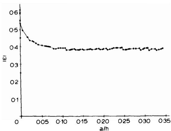
Fig. 10. \varepsilon - a curve for a (0, \pm 45, 90)_s laminate: delamination on the mid-plane interface.
