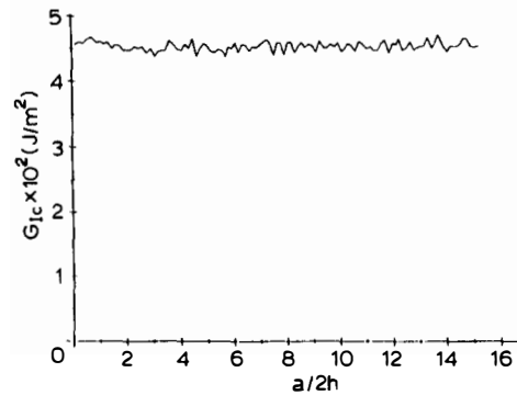
Fig. 9. G_{Ic}-a curve.
