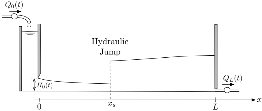
Figure 1: Open channel with a hydraulic jump and three control devices : the gate opening H_0(t) and the inflow Q_0(t) and outflow Q_L(t) which are driven by two pumps.
