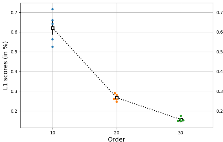
Figure 3: L_1 scores computed according to (29). Each dot is an estimated value with the least squares approach. For each value of r , the mean value (squares) over all runs as long as the empirical standard deviation (bars) are displayed.
