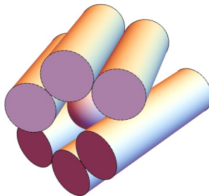
Figure 4: Non-rigidity of C_6
