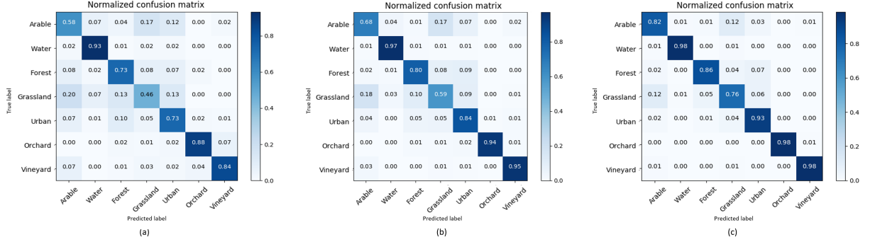
Fig. 8: Normalized confusion matrix for the best results obtained with AlexNet on the class-balanced subset. a) 25 pixels \times 25 pixels; b) 50 pixels \times 50 pixels; c) 100 pixels \times 100 pixels.
