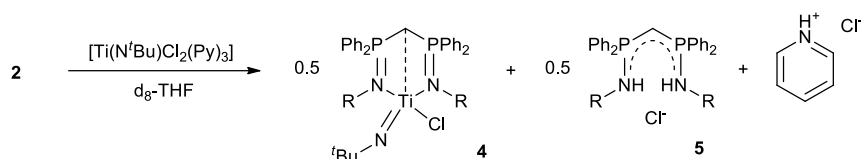
Scheme 2 Formation of BIPMH Ti-imido complex 4
