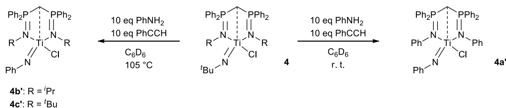
Scheme 5 In situ formation of Ti=NPh species
