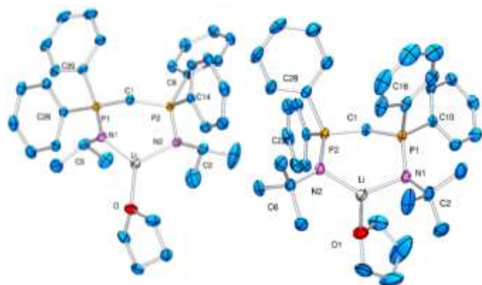
Fig. 3 POV-RAY depiction of 3b and 3c (thermal ellipsoids drawn at the 50 % probability level)
