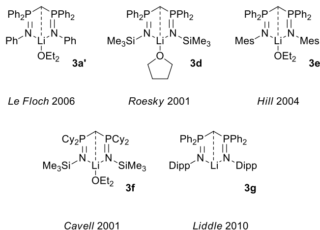
Fig. 4 Structurally characterized monomeric Li complexes 10, 15, 45-47
