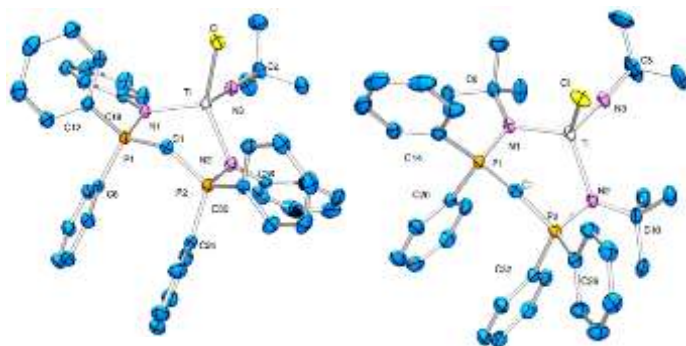
Fig. 5 POV-RAY depiction of 4a and 4c (thermal ellipsoids drawn at the 50 % probability level)
