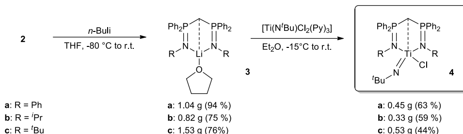
Scheme 3 Synthesis of BIPMH-stabilized Ti-imido complexes by transmetalation with Li complexes
