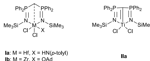
Fig. 2 Relevant group 4 BIPMH and BIPM complexes reported by Cavell 18
