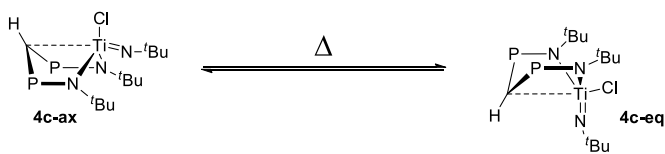
Scheme 4 Dynamic equilibrium between the two boat isomers of 4c
