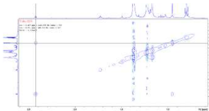
Fig. 6 EXSY NMR, high field region (500 MHz, CD 2 Cl 2 , 323 K, 300 ms mixing time) 54
