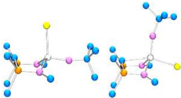
Fig. 7 Calculated structures for 4c-ax (left) and 4c-eq (right). Ph and t Bu groups on the BIPMH ligand removed for clarity
