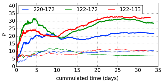
Figure 4. Convergence of the noise correlation function for three pairs of nodes in the EstOF network (220–172, 122–172, and 122–133). The ratio ( R ) between the peak amplitude in the direct arrival window (group velocity between 0.3 and 3.5 km/s) and the coda window (group velocity between 0.15 and 0.3 km/s) is measured for both causal (thick curves) and acausal sides (thin curves).
