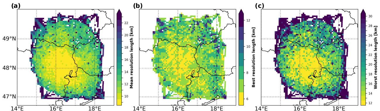
Figure 7. Resolution analysis of the group-velocity inversion for 15 s centre period. (a) Mean resolution length of the resolution matrix of each cell. (b) Resolution length in the best direction, i.e. the best resolution length. (c) Resolution length in the worst direction, i.e. the worst resolution length.
