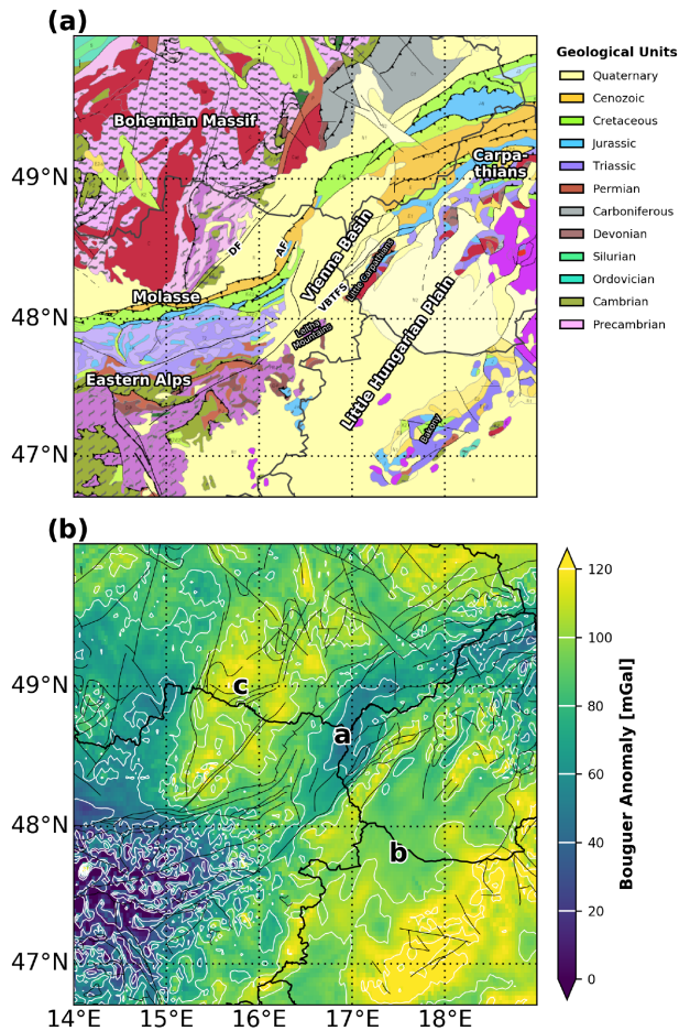
Figure 13. (a) Surface geology of the study area extracted from the International Geological Map of Europe (IGME5000; Aschk 2005). Major features are labelled. Shown faults (black lines) are combined from the IGME5000 and the EDSF (Basili et al. 2013). (b) Bouguer gravity anomaly in the study area, extracted from the World Gravity Map 2012 (WGM2012; Bonvalot et al. 2012). Labelled features: Vienna Basin (a); Little Hungarian Plain (b); Bohemian Massif (c).
