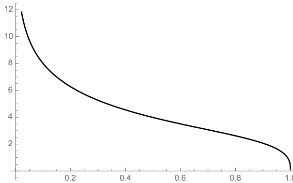
FIGURE 2. The period T_a of the solution of (12) with initial datum X(0) = a \in (0, 1) and Y(0) = 0 as a function of a for p = 3 and q = 5 . We observe that \lim_{a \rightarrow 0} T_a = +\infty and \lim_{a \rightarrow 1} T_a = 0 .
