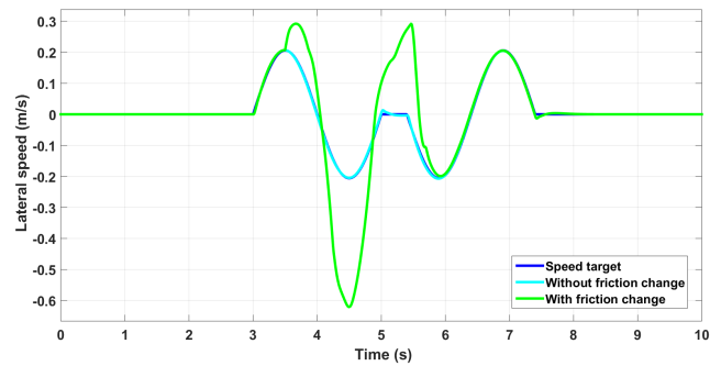
Fig. 4. Lateral speed control when vertical dynamics are considered.
