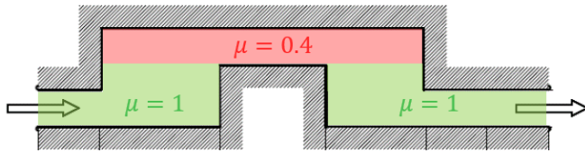
Fig. 1. ISO 3888-1:1999(E) standard with friction variation.
