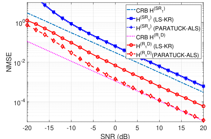
Fig. 11. CRBs for the channels \mathbf{H}^{(SR_1)} and \mathbf{H}^{(R_1 D)} and their respective NMSE generated by LS-KR and PARATUCK-ALS, for K = 1 .
