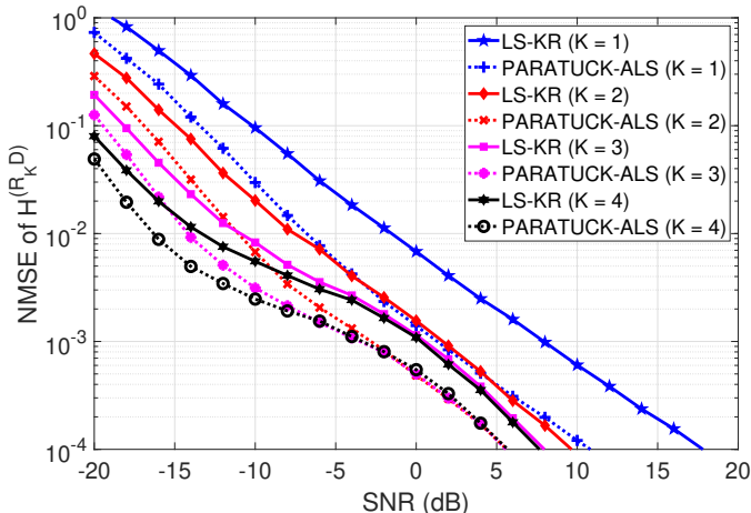
Fig. 9. NMSE of \mathbf{H}^{(R_K D)} versus SNR for the LS-KR and PARATUCK-ALS receivers, for several values of K .
