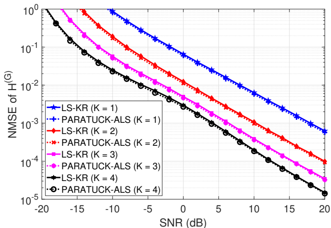
Fig. 7. NMSE of \mathbf{H}^{(G)} versus SNR for the LS-KR and PARATUCK-ALS receivers, for several values of K .
