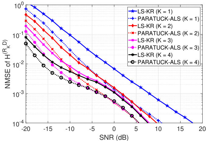
Fig. 8. NMSE of \mathbf{H}^{(R_K D)} versus SNR for the LS-KR and PARATUCK-ALS receivers, for several values of K .
