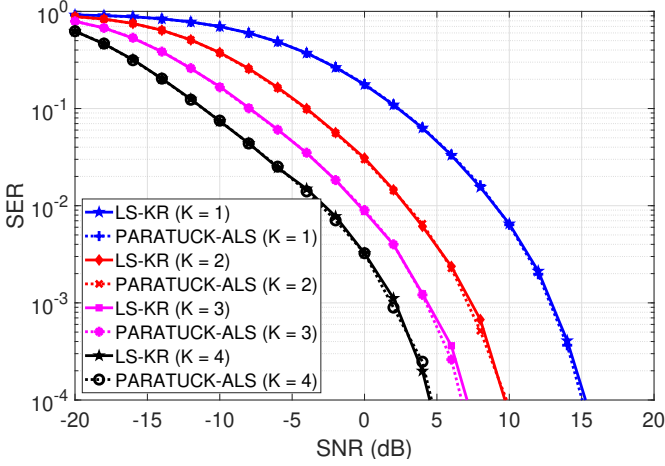
Fig. 4. SER versus SNR for the LS-KR and PARATUCK-ALS receivers, for several values of K .
