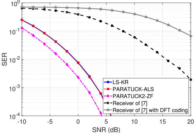
Fig. 3. SER versus SNR for the LS-KR, PARATUCK-ALS, PARATUCK2-ZF receivers and the receiver of [7] using its original Vandermonde matrix coding and the DFT coding used in the proposed receivers.
