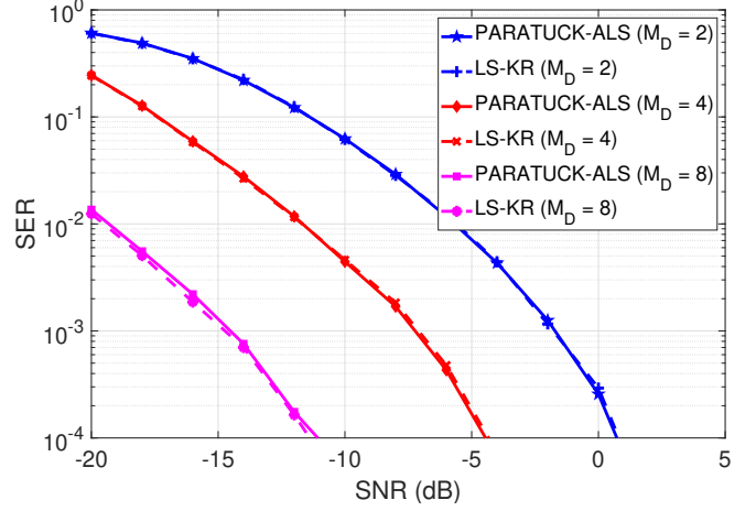
Fig. 5. SER versus SNR varying the number of antennas at the destination for the LS-KR and PARATUCK-ALS receivers.
