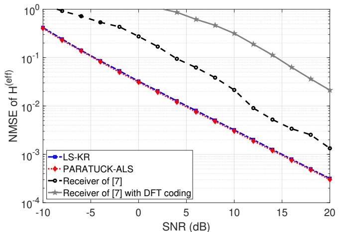
Fig. 9. NMSE versus SNR for the effective channel \mathbf{H}^{(eff)} for the LS-KR, PARATUCK-ALS receivers and the receiver of [7] using its original Vandermonde matrix coding and the DFT coding used in the proposed receivers.
