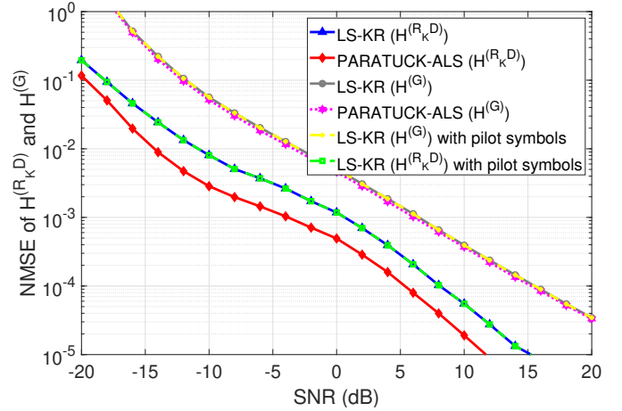
Fig. 6. NMSE versus SNR for \mathbf{H}^{(R_K D)} and \mathbf{H}^{(G)} for the LS-KR and PARATUCK-ALS receivers, for K = 3 .
