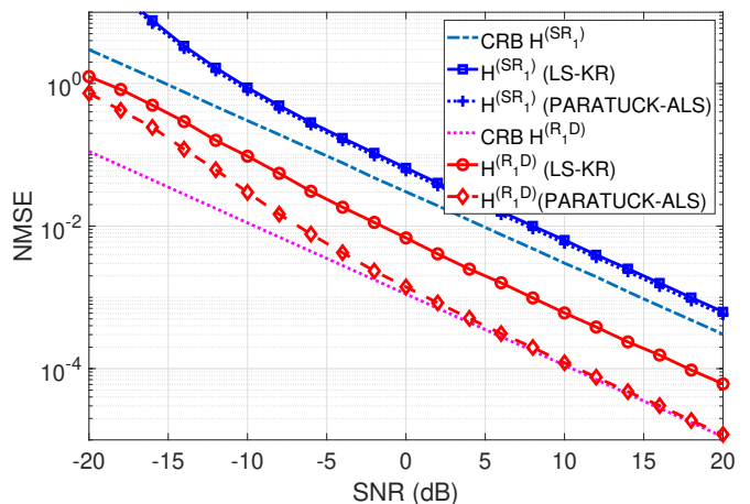
Fig. 11. CRBs for the channels \mathbf{H}^{(SR_1)} and \mathbf{H}^{(R_1^D)} and their respective NMSEs generated by LS-KR and PARATUCK-ALS, for K = 1 .
