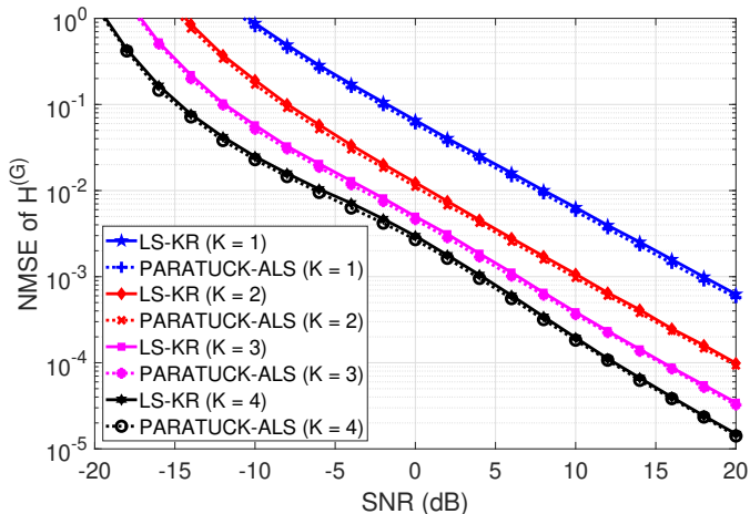
Fig. 8. NMSE of \mathbf{H}^{(G)} versus SNR for the LS-KR and PARATUCK-ALS receivers, for several values of K .
