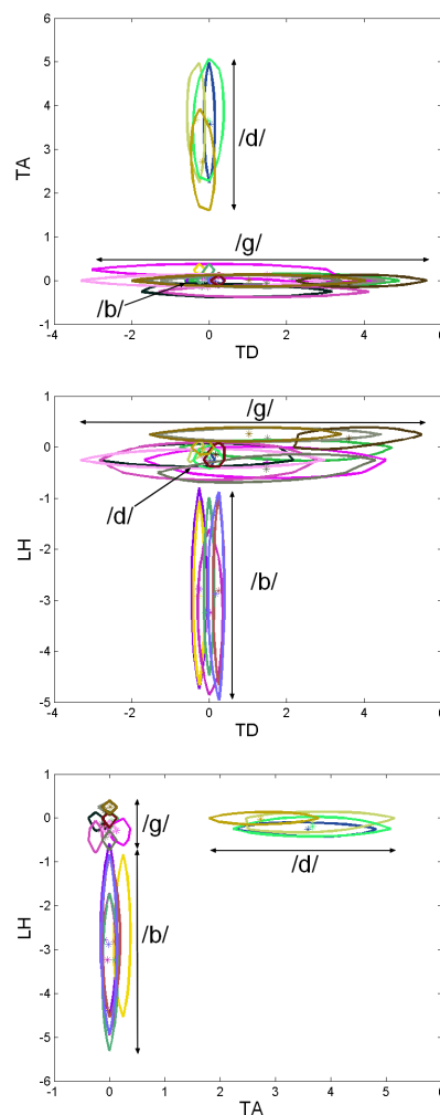
Figure 4: Illustration of consonantal Gaussian distributions for significant kernels (with prior probability > 0.01 ), in the dimensions TD , LH and TA of the motor space \Delta M . Each ellipse with one color represents the same Gaussian distribution in the three sub-plots.
