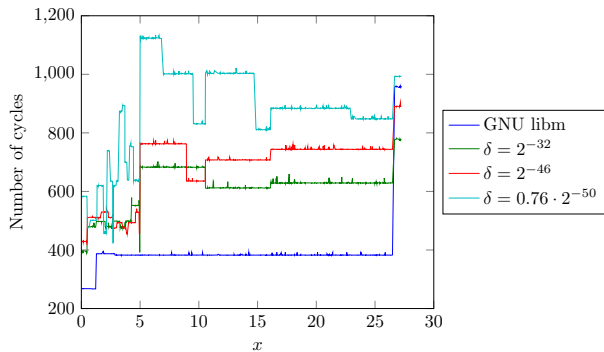
Fig. 4. Performance comparison without compiler optimization (-O0).
