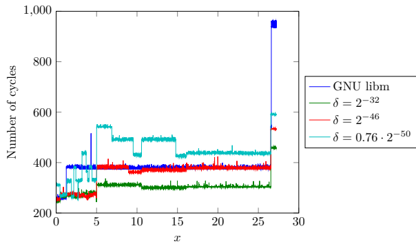
Fig. 3. Performance comparison with maximum compiler optimization (-O3).
