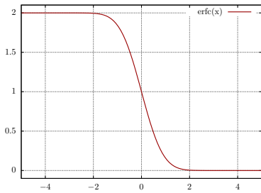
Fig. 1. Function \text{erfc} for input arguments in [-5; 5] .
