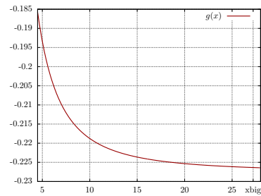
Fig. 2. Function g(x) for x \in [5; x_{\text{BIG}}] .
