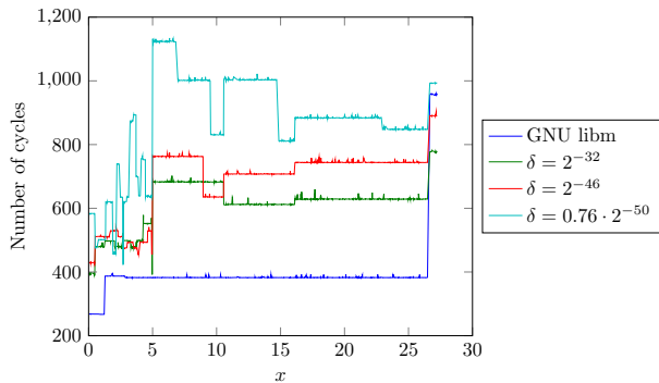
Fig. 4. Performance comparison without compiler optimization (-O0).
