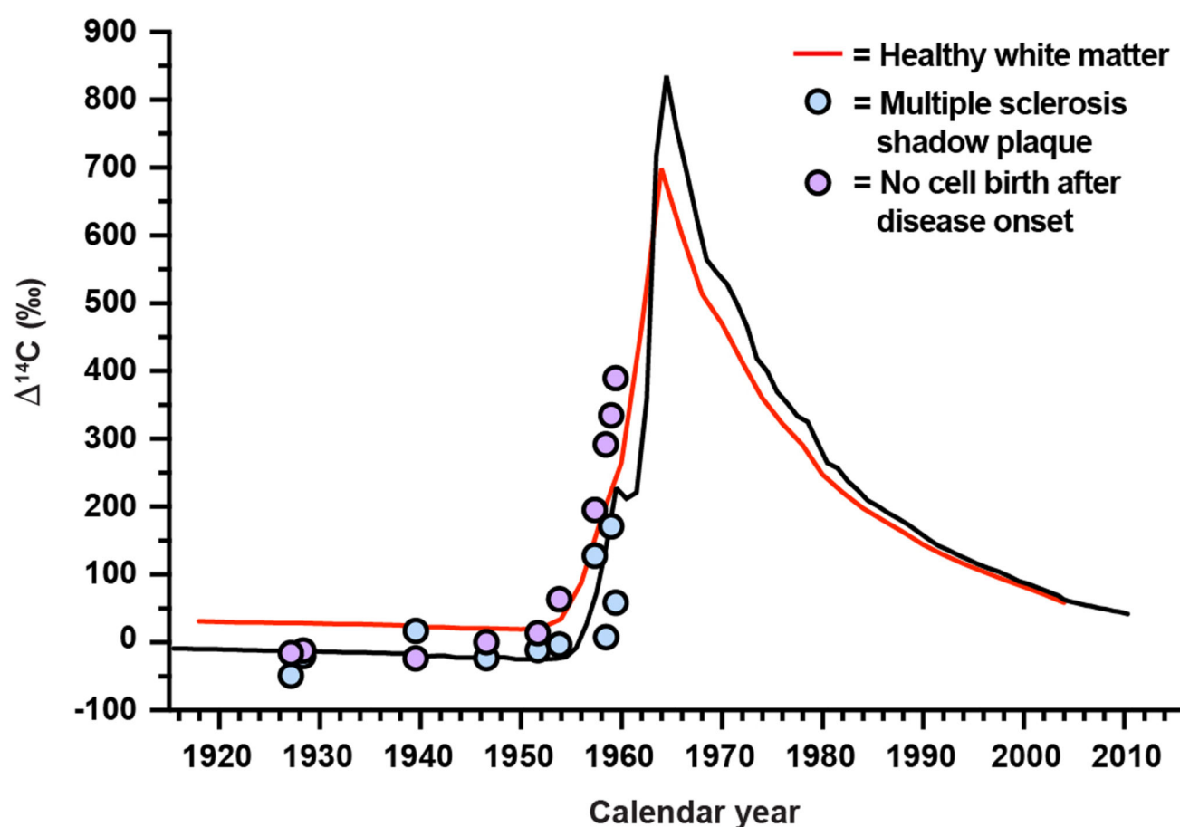
Extended Data Figure 4. Modeled ^{14}\text{C} concentration in DNA of oligodendrocytes generated until disease onset
