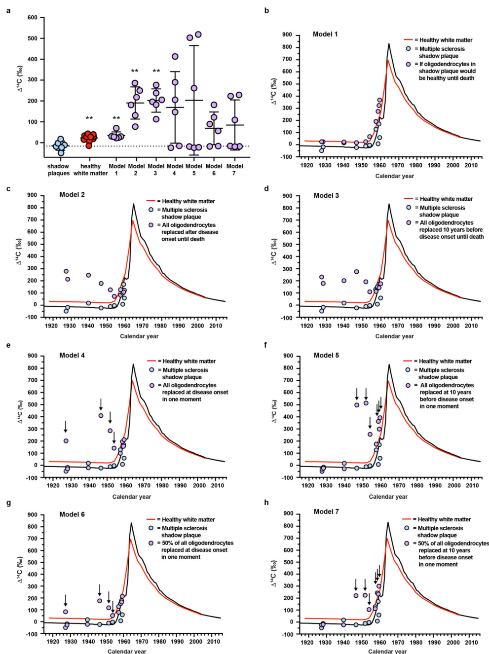
Extended Data Figure 8. Modeled ^{14}\text{C} concentration in DNA of oligodendrocytes generated from oligodendrocyte progenitor cells in shadow plaques
