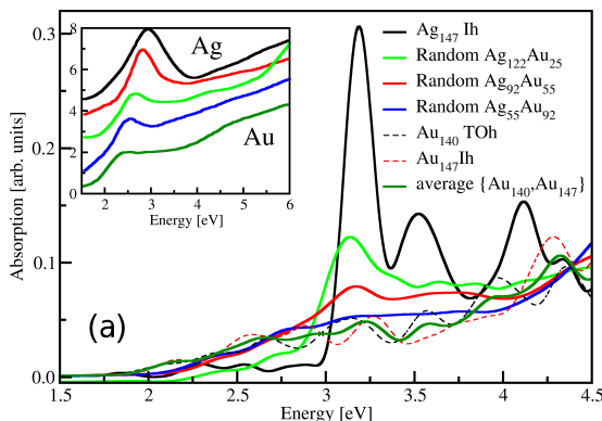
Figure 5 – Absorption spectra of 147-atom icosahedral Ag-Au random alloy clusters, compared with the experimental results of Gaudry et al. [60] shown in the inset for compositions x = 0.00, 0.25, 0.50, 0.75, and 1.00 . Figure taken from [61].
