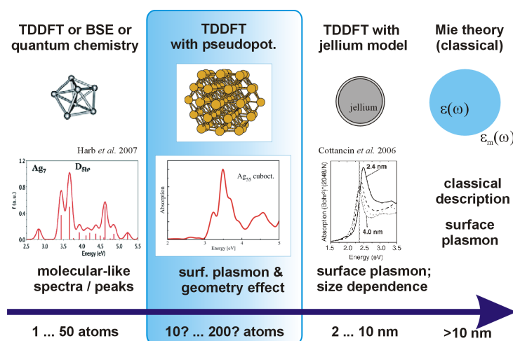
Figure 1 – Illustration of the different size ranges exhibiting different types of spectra, being dominated by different effects, and calling for different theoretical descriptions. The size-dependence of the LSPR in the inset is taken from Ref. [2].
