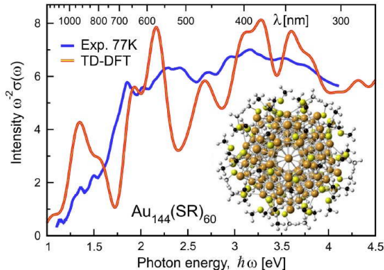
Figure 4 – Optical spectra for the ubiquitous icosahedral gold clusters, \text{Au}_{144}(\text{SR})_{60} . Theory (red) and experiment (blue). Plotted is the optical absorption cross-section frequency-weighted to match the optical-absorbance function. Figure taken from [10] and its Supplementary Material.
