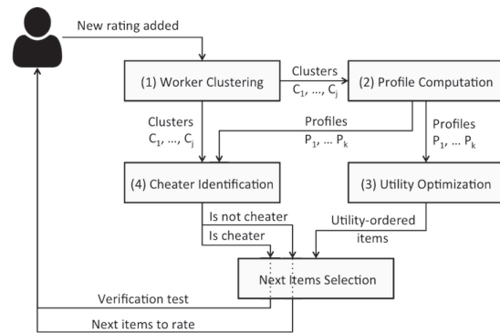
Figure 1: The Crowdsourcing Platform.
