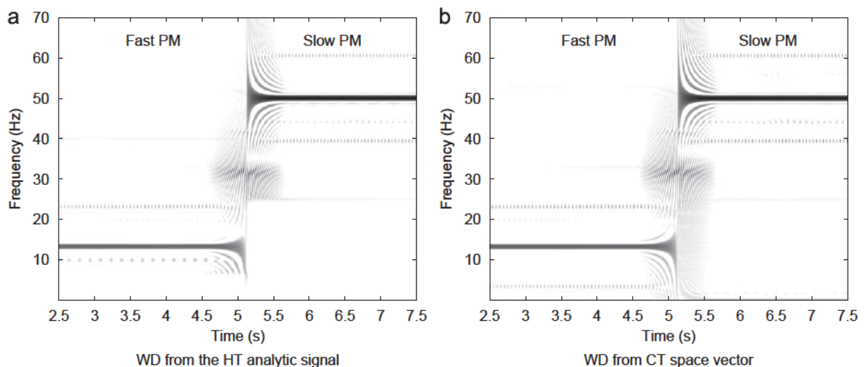
Fig. 7. WD computed using HT and CT for fast and slow PM experimental currents in steady state. (a) WD from the HT analytic signal. (b) WD from CT space vector.
