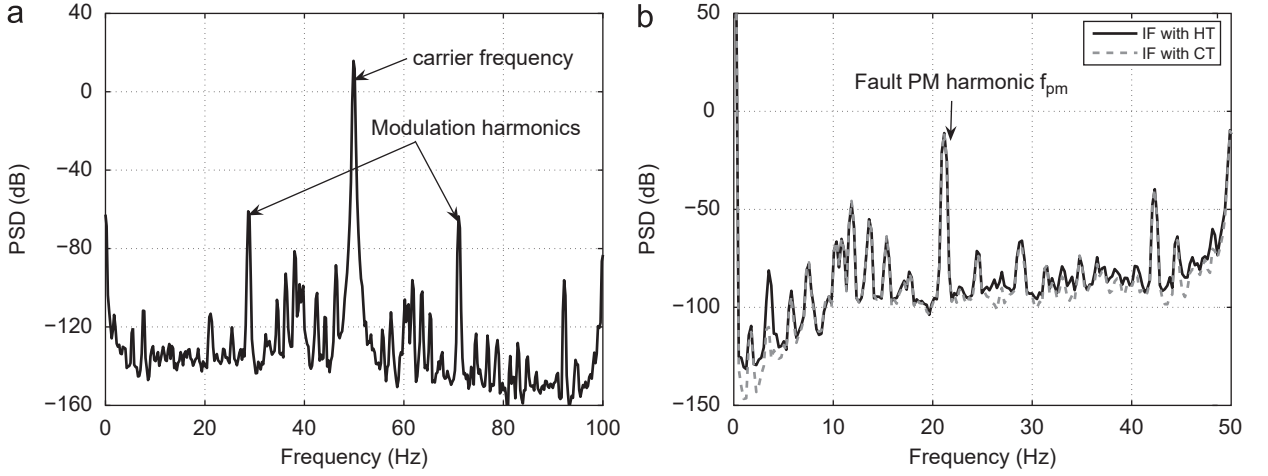
Fig. 4. Spectrum of stator current and associated IF computed through the HT and CT in case of slow PM.
