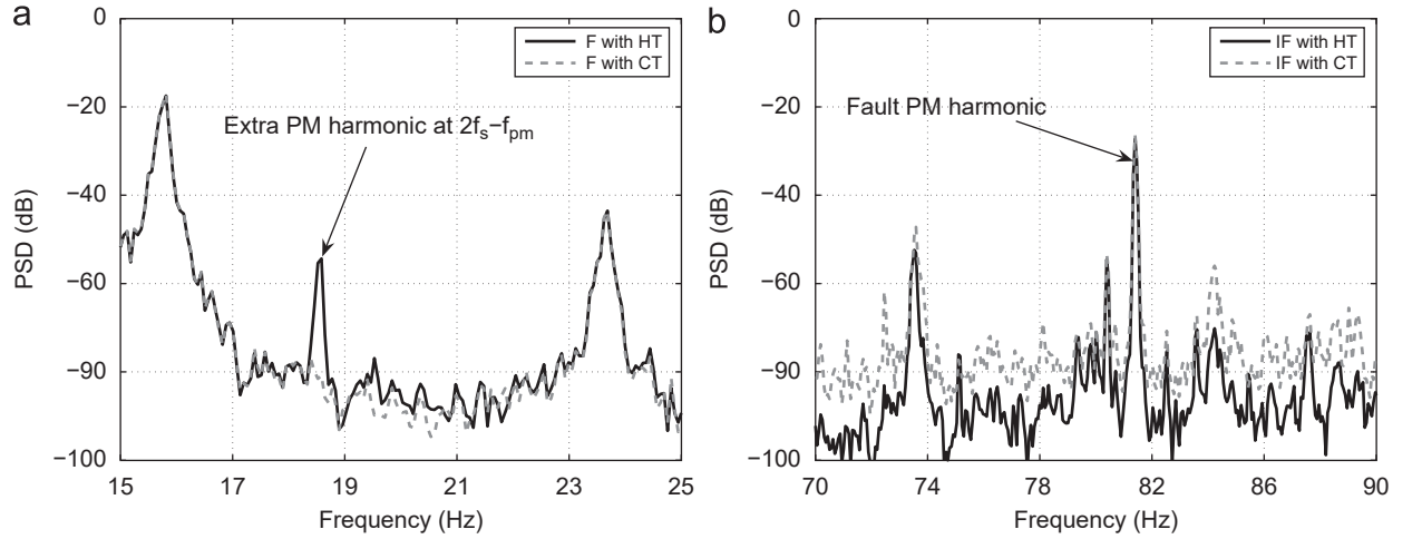
Fig. 6. Spectrum of IF computed through the HT and CT in case of fast PM.
