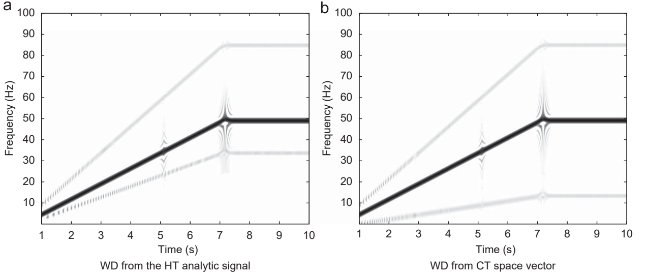
Fig. 8. WD from HT and CT for simulated fast PM at variable speed. (a) WD from the HT analytic signal. (b) WD from CT space vector.
