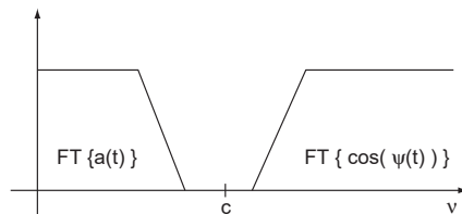
Fig. 1. Illustration of the Bedrosian theorem conditions.
