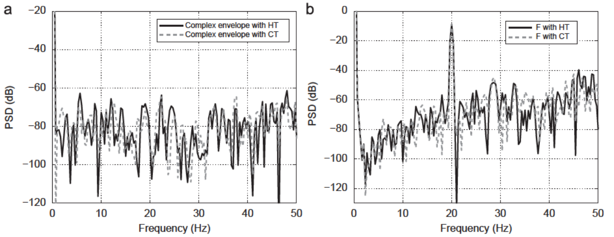
Fig. 3. Spectrum of IA and IF computed through the HT and CT in case of slow PM.
