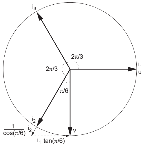
Fig. 2. Geometrical construction of the Concordia basis from the three current components.
