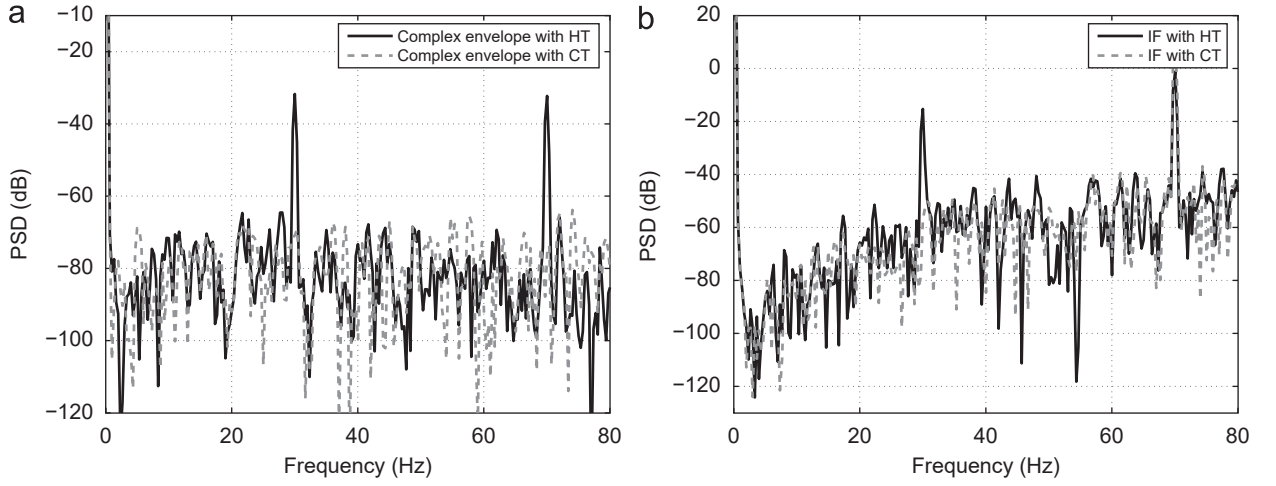
Fig. 5. Spectrum of simulated complex envelope and instantaneous frequency computed through the HT and CT in case of fast PM.
