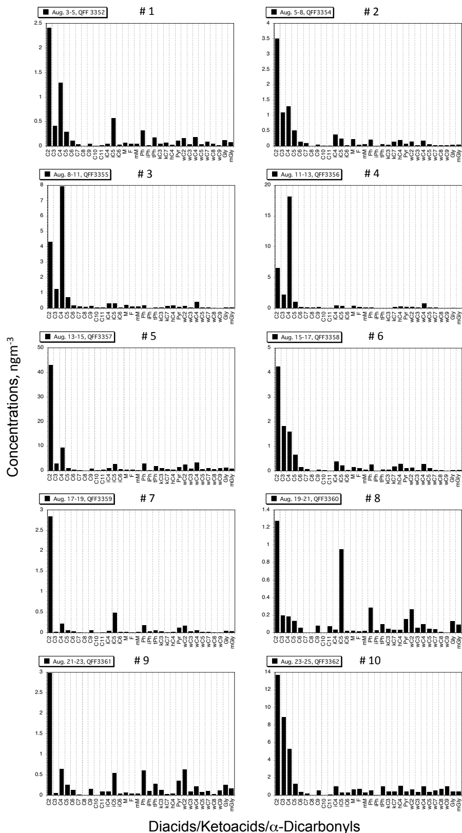
Fig. 4. Molecular compositions of low molecular weight dicarboxylic acids (C 2 –C 10 ), ketocarboxylic acids (C 2 –C 9 ) and \alpha -dicarbonyls (glyoxal and methylglyoxal) in the Arctic marine aerosols. For the details of samples #1–#10, see Fig. 1. For the abbreviations of compounds, see Table 1.
