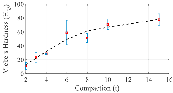
Fig. 14. Vickers Hardness number as a function of the compaction of the JSC1 targets. The error bars give the standard deviation of the five measurements performed on each target.
