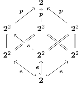
FIGURE 13.1. The commutative diagram \vec{S}
