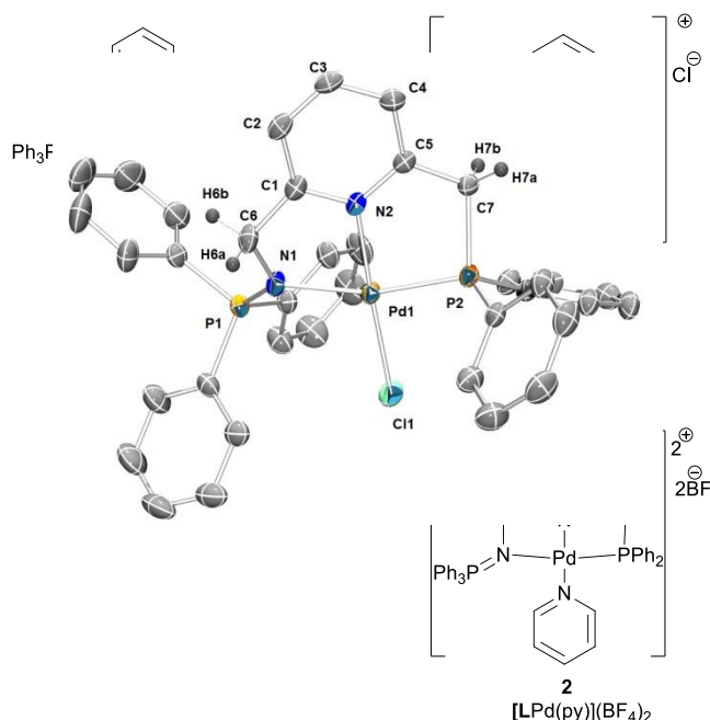
Figure 2: ORTEP of the solid-state structure of 1 with 50% probability thermal ellipsoids. Most Hydrogen atoms, one non-coordinating chloride and one benzonitrile solvent molecule were omitted for clarity. Selected bond lengths [ \text{\AA} ] and angles (deg): N1-P1 1,603(2), N1-Pd1 2,110(2), P2-Pd1 2,212(7), N2-Pd1 1,998(2), Cl1-Pd1 2,2953(7); N1-Pd1-P2 164,23(6), N2-Pd1-Cl1 175,95(6), N1-Pd1-N2 80,2(1), P2-Pd1-N2 84,04(6), N1-Pd1-Cl1 99,9(2), P2-Pd1-Cl1 93,19(3).
