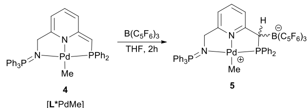
Scheme 6: Formation of 5
