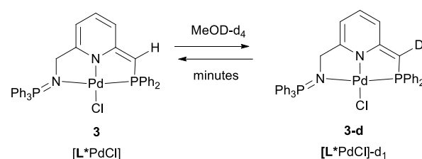
Scheme 5: Reactivity of [L^*PdCl](3) with deuterated methanol
