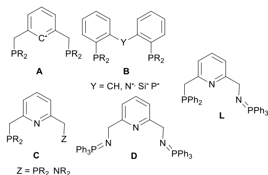
Figure 1: Pincer phosphine and/or iminophosphorane ligands
