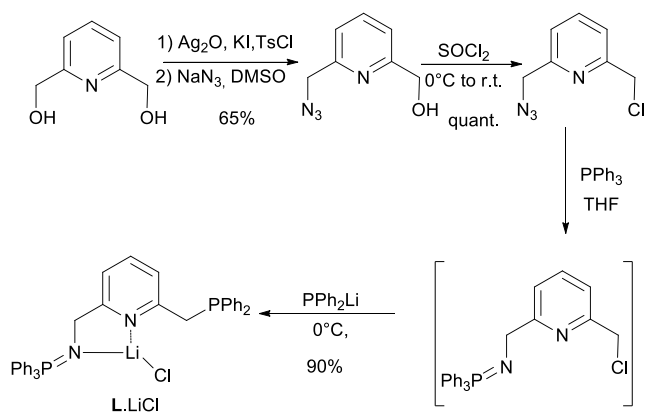
Scheme 1: Synthesis of L .LiCl
