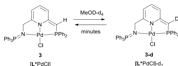
Scheme 5: Reactivity of [L^*PdCl](3) with deuterated methanol
