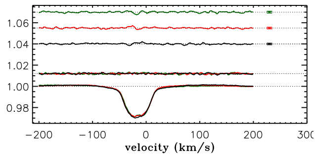
Fig. B.14. LSD profiles for IRAS 22144 + 6923 (magnetic field detected, complex topology).
