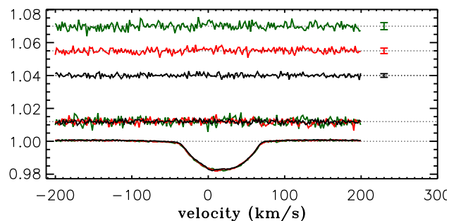
Fig. B.16. LSD profiles for NGC 2264 108 (no magnetic detection).
