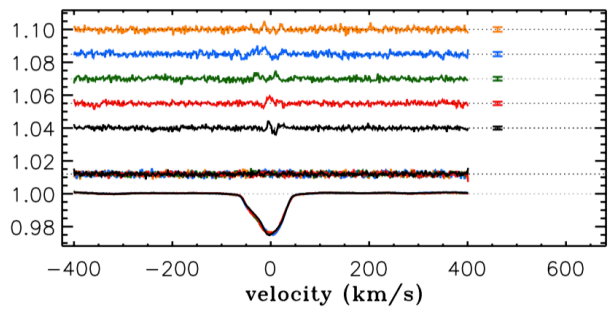
Fig. B.36. LSD profiles for V 1156 Sco (magnetic field detected, complex topology).
