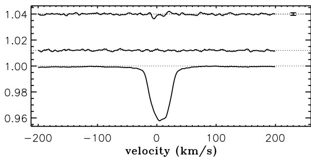
Fig. B.9. LSD profiles for HD 133938 (magnetic field detected, complex topology).
