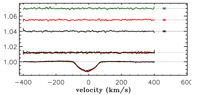
Fig. B.29. LSD profiles for PX Vul (no magnetic detection).
