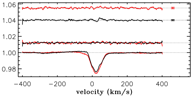
Fig. B.3. LSD profiles for CO Ori (magnetic field detected, uncertain topology).
