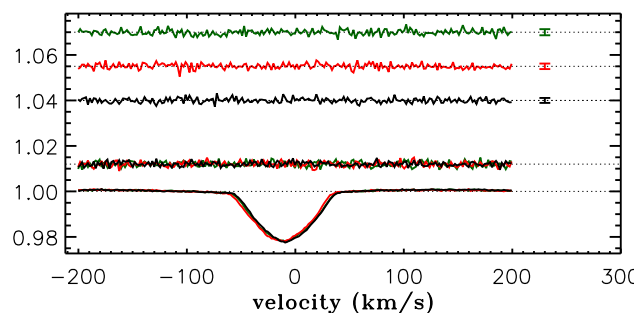
Fig. B.15. LSD profiles for IRAS 22152 + 6947 (no magnetic detection).
