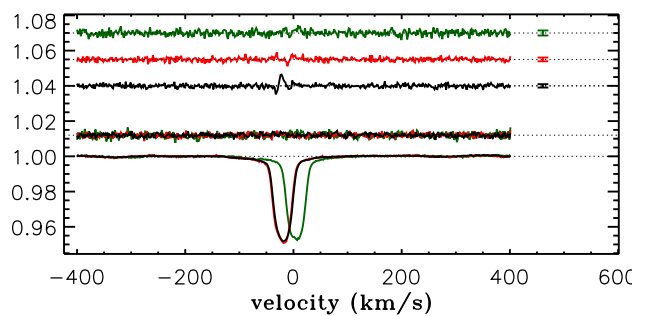
Fig. B.32. LSD profiles for V 1001 Sco (magnetic field detected, complex topology).
