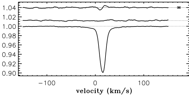
Fig. B.2. LSD profiles for CHX 22 (magnetic field detected, simple topology).
