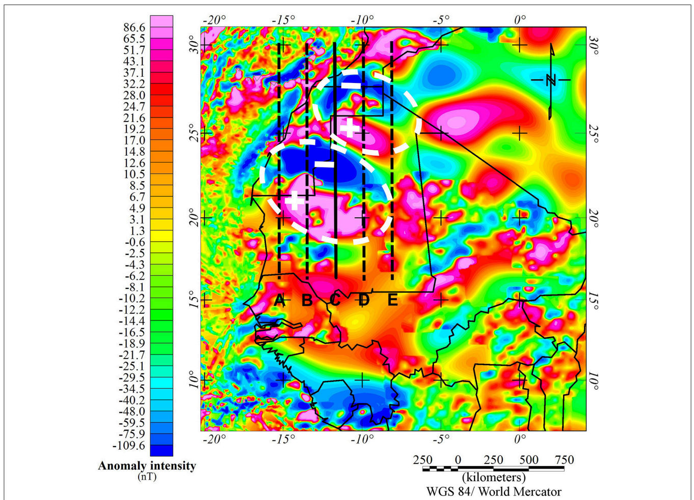
FIGURE 1 | The West Africa Magnetic Anomaly (WAMA) in the World Digital Magnetic Anomaly Map (WDMAM) model at 5 km altitude. Segments A–E correspond to the selected profiles used for 2D modeling. Solid segment C corresponds to the profile shown in this article.
