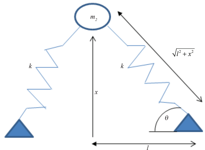
Figure 5 – Simplified movement model of the NES
