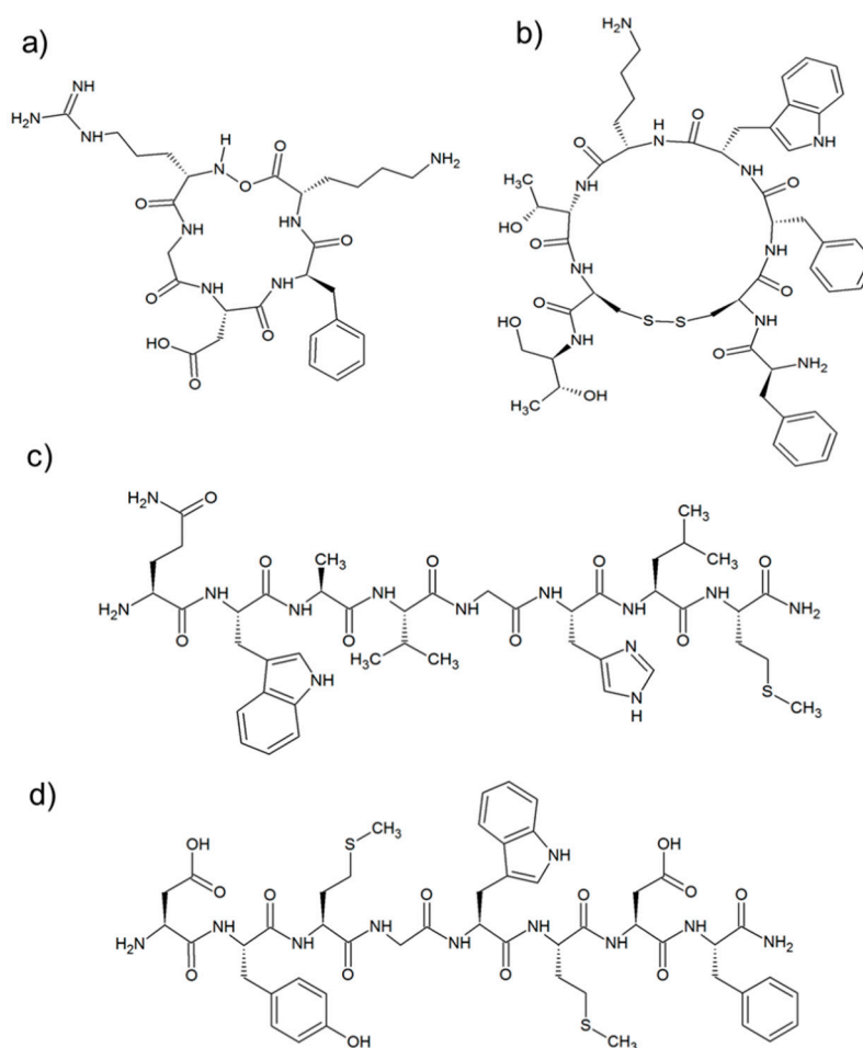
Figure 4. Structure of targeting peptide sequences: (a) c(RGDfK); (b) Otreotide[c(2–7)-FCFWKTCTol]; (c) [7–14]-Bombesin (H-QWAVGHLM-NH 2 ), and (d) CCK8(H-DYMGWMDF-NH 2 ).
