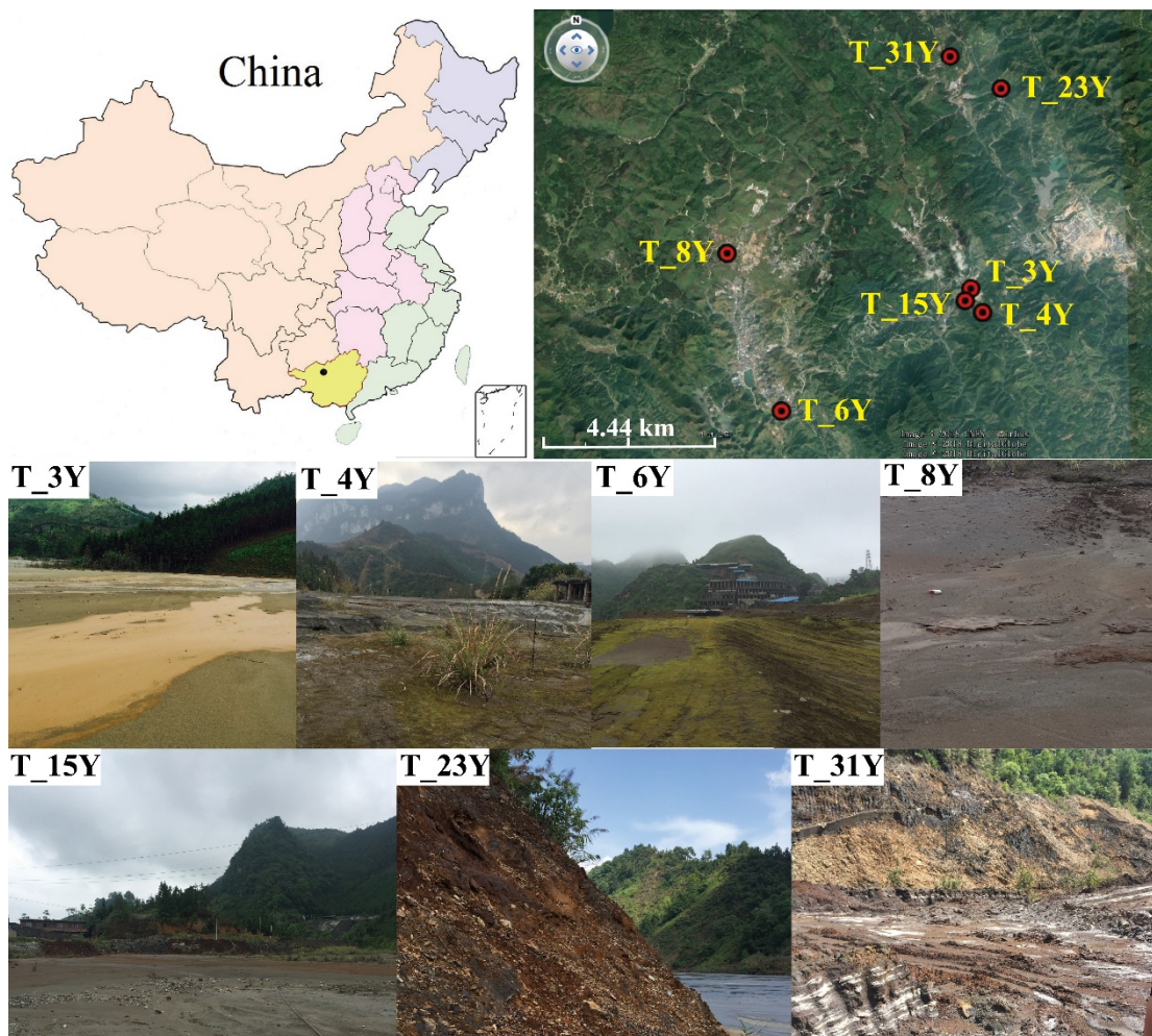
715 Fig. 1. Sample location map (top left) and aerial photograph (top right) of the seven 716 tailings sites (T_3Y to T_31Y) close to Hechi city (● shown on map), Guangxi 717 (China), where the surface samples (● on aerial photo) were collected for the present 718 study. Field photographs of tailing sample sites are shown in the bottom panels (T_3Y 719 to T_31Y). As an example, T_3Y corresponds to the tailing sample code. T_3Y 720 means the tailing samples were taken from a three years old abandoned site (not-used).
